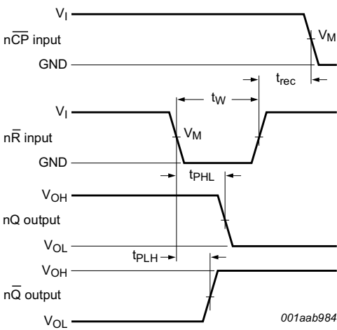
Measurement points are given in Table 8 . V_{OL} and V_{OH} are typical voltage output levels that occur with the output load.
