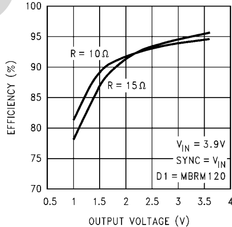
Efficiency vs Output Voltage (PWM MODE, with Diode)
