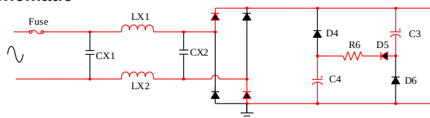
Figure 8: Stage B of Valley Fill Circuit
