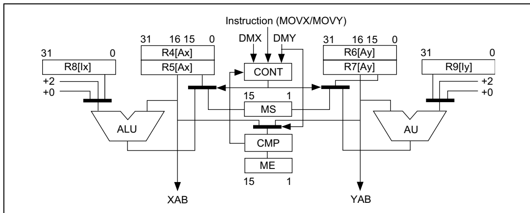
Figure 2.14 Modulo Addressing
