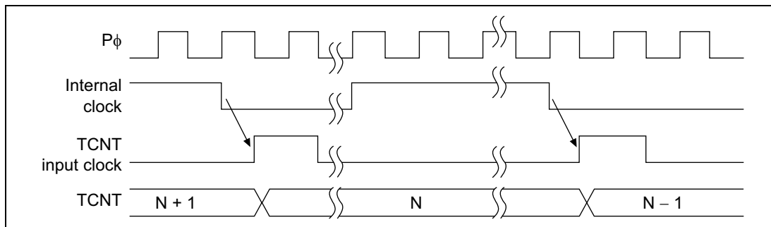
Figure 13.4 Count Timing when Operating on Internal Clock
