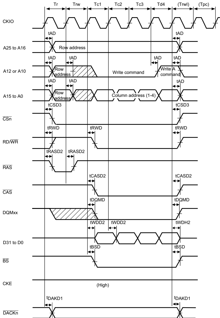
Figure 24.29 Synchronous DRAM Write Bus Cycle (Burst Mode (Single Write \times 4 ), RCD = 1, TPC = 0, TRWL = 0)
