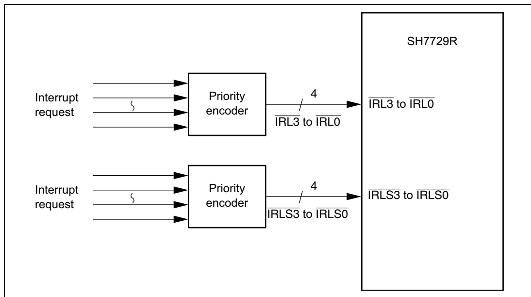
Figure 7.2 Example of IRL Interrupt Connection
