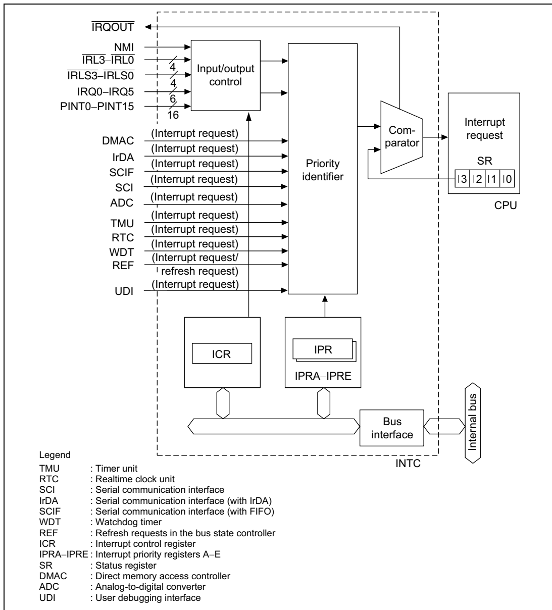
Figure 7.1 Block Diagram of INTC
