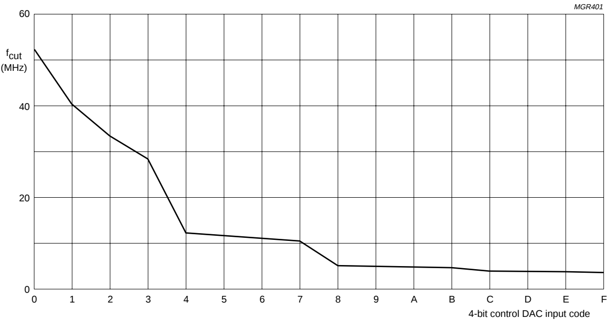
Fig.13 AGC bandwidth.
