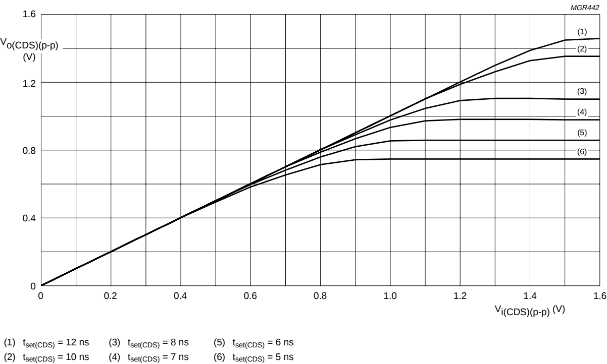
Fig.14 CDS output.
