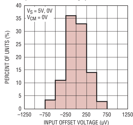
V_{OS} Distribution, V_{CM} = 0\text{V} (SOT-23, PNP Stage)
