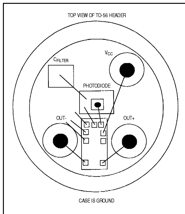
Figure 3. Suggested Layout for TO-56 Header
