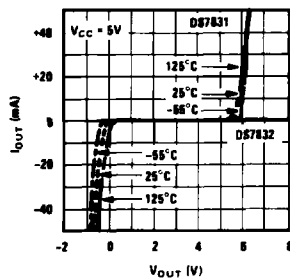
I OUT vs V OUT High Impedance Output State
