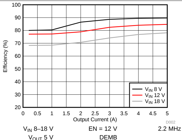
Figure 2. Efficiency vs I_{OUT}
