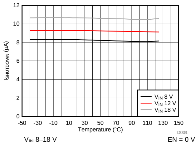
Figure 4. I_{SHUTDOWN} vs Temperature
