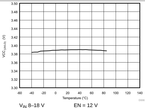
Figure 6. V_{CC(UVLO)} vs Temperature
