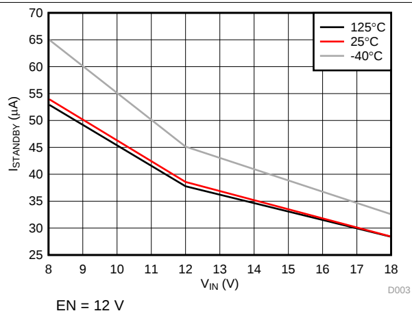
Figure 3. I_{STANDBY} vs V_{IN}
