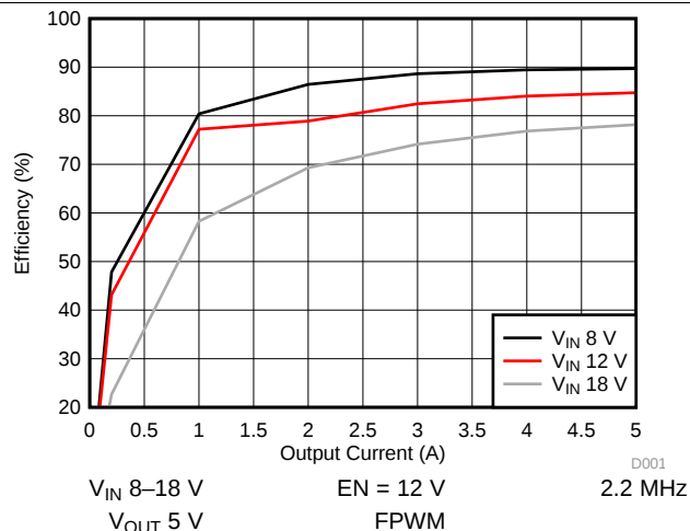
Figure 1. Efficiency vs I_{OUT}
