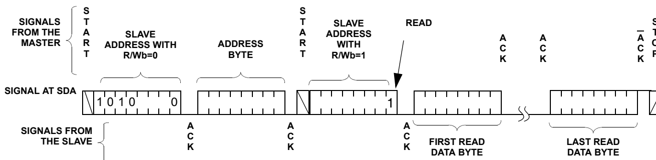
FIGURE 10. READ SEQUENCE
