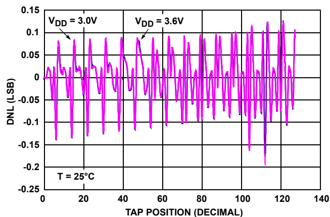
FIGURE 3. DNL vs TAP POSITION FOR 10kΩ (W)
