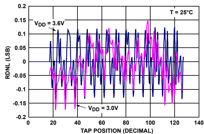
FIGURE 5. RDNL vs TAP POSITION FOR 10kΩ (W)
