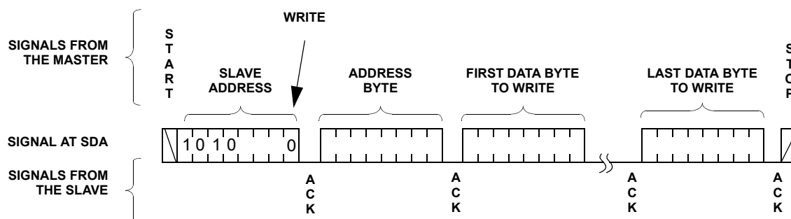
FIGURE 9. WRITE SEQUENCE
