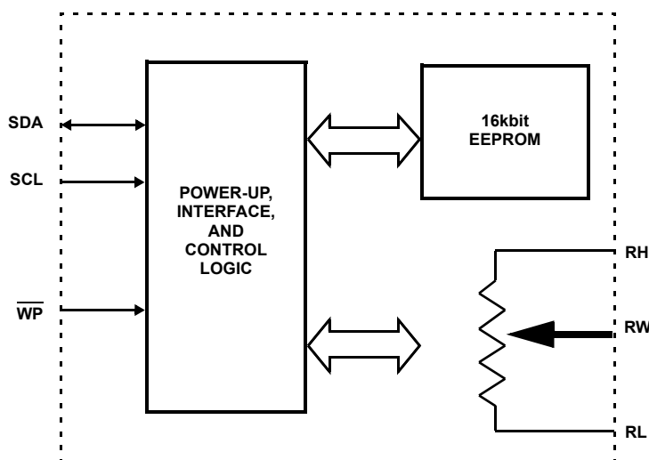
FIGURE 1. BLOCK DIAGRAM
