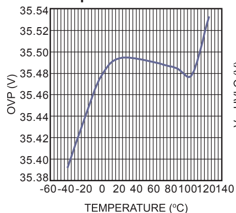
OVP Voltage vs. Temperature
