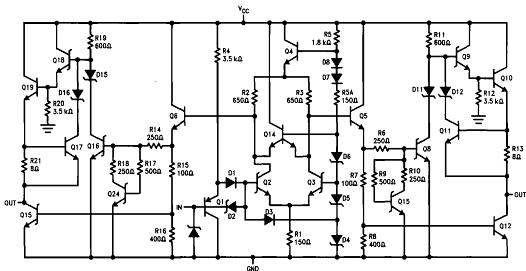
FIGURE 1. Equivalent Circuit
