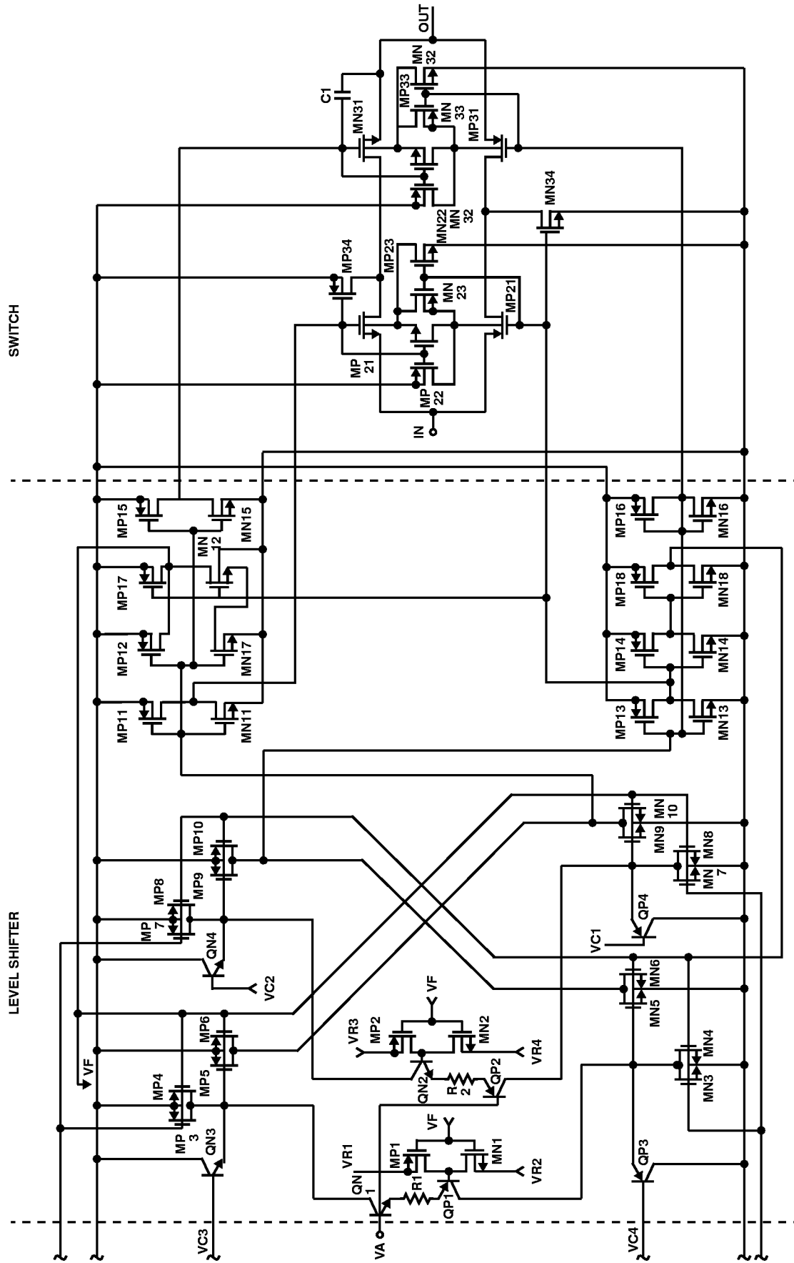
Schematic Diagram (Continued)
