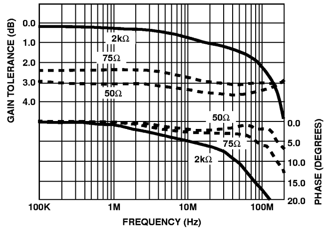
FIGURE 13. BANDWIDTH
