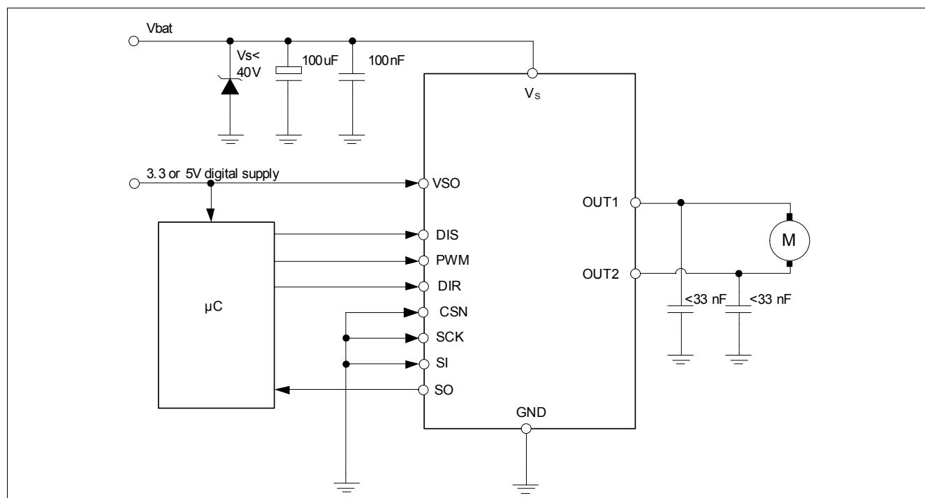
Figure 11 Application Example H-Bridge with Error Flag
