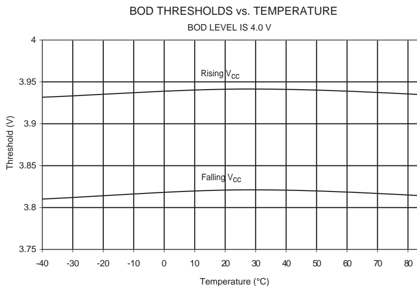
Figure 198. BOD Thresholds vs. Temperature (BODLEVEL is 4.0V)
