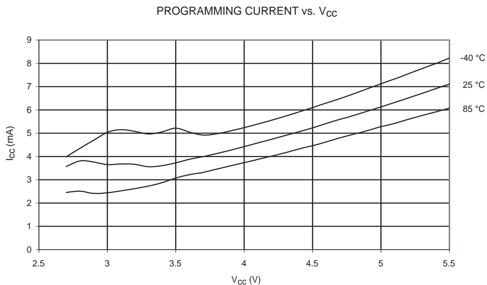
Figure 218. Programming Current vs. V_{CC}
