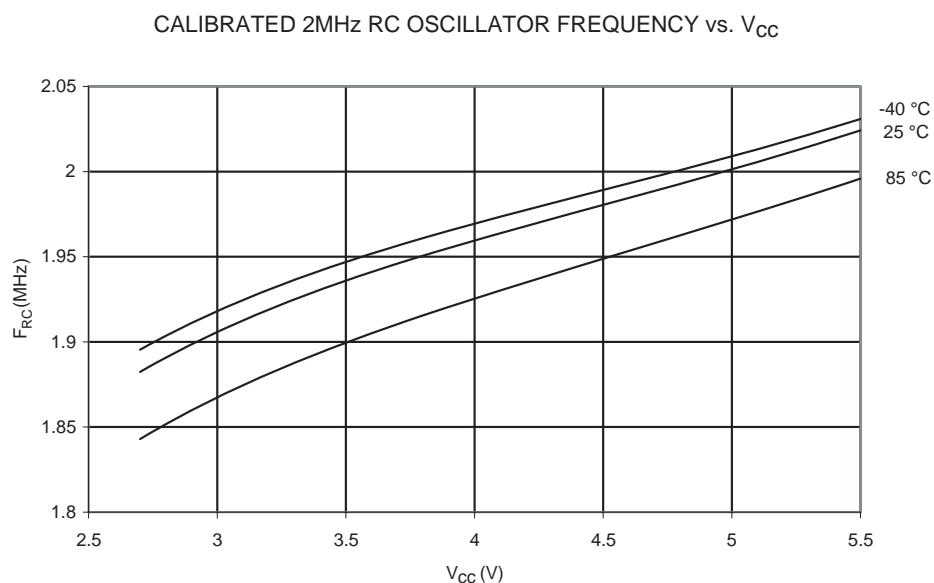
Figure 206. Calibrated 2 MHz RC Oscillator Frequency vs. V_{CC}
