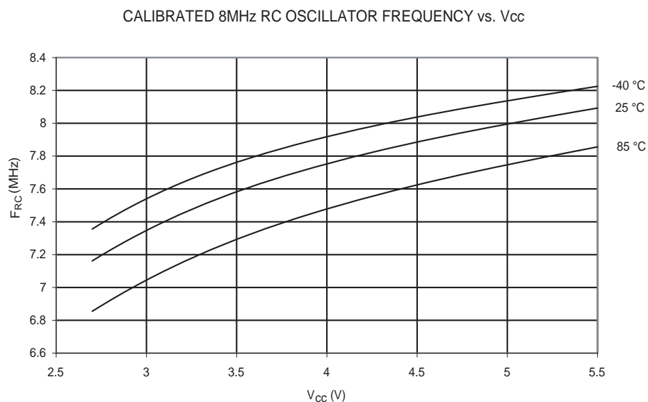
Figure 212. Calibrated 8 MHz RC Oscillator Frequency vs. V_{CC}
