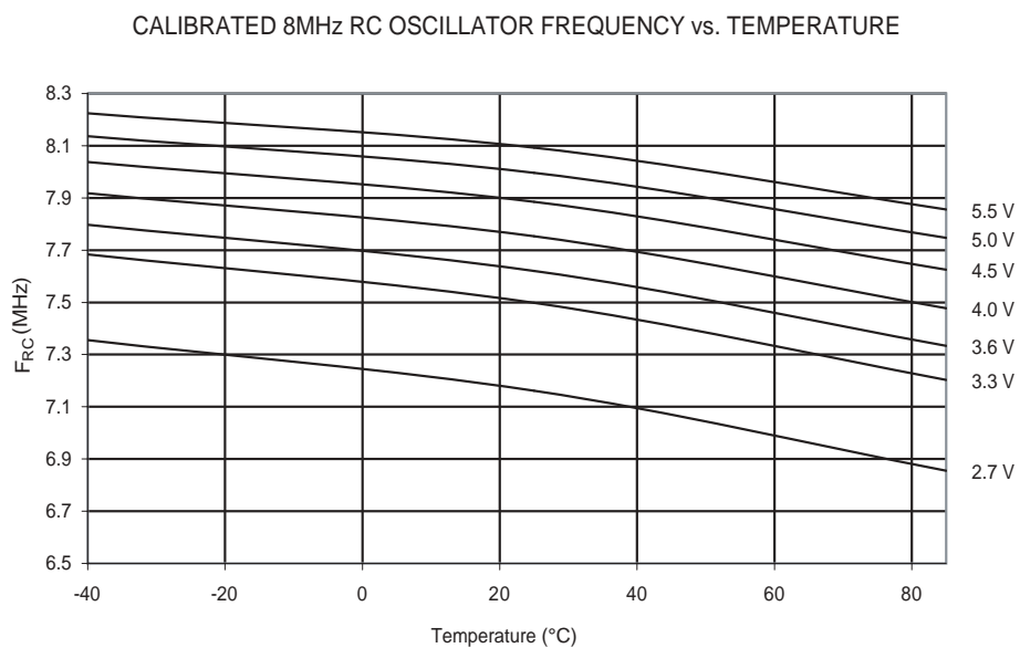
Figure 211. Calibrated 8 MHz RC Oscillator Frequency vs. Temperature
