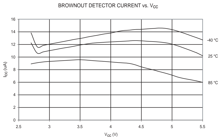
Figure 214. Brownout Detector Current vs. V_{CC}
