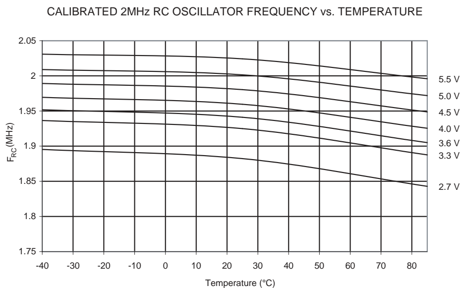
Figure 205. Calibrated 2 MHz RC Oscillator Frequency vs. Temperature
