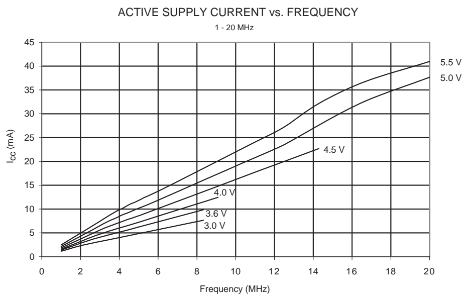
Figure 164. Active Supply Current vs. Frequency (1 - 20 MHz)
