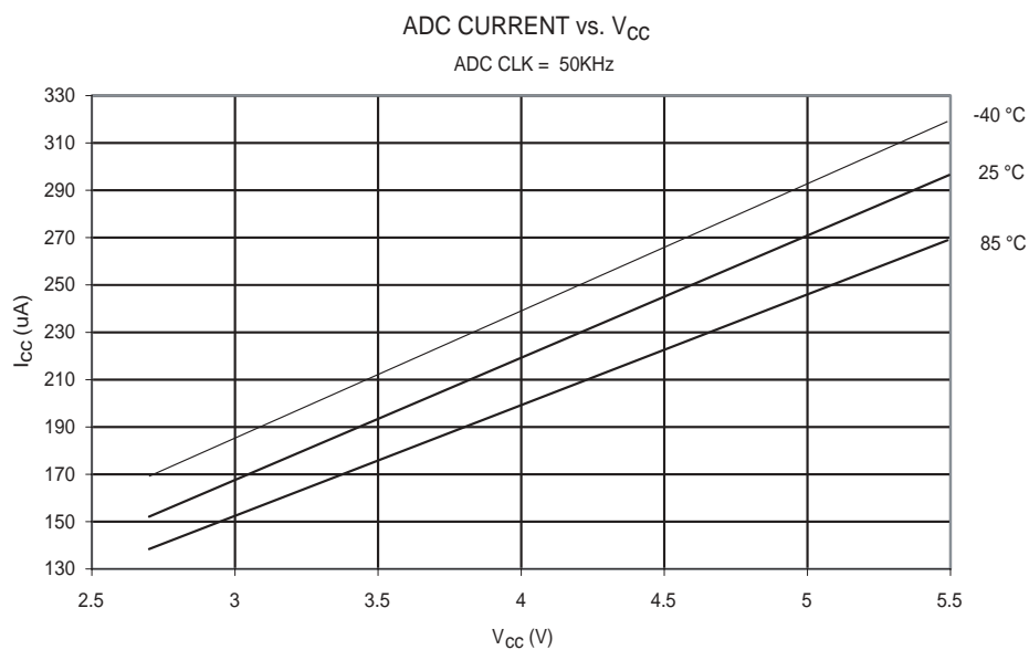
Figure 215. ADC Current vs. V_{CC} (ADC CLK = 50 kHz)
