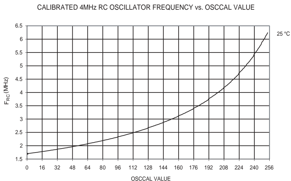
Figure 210. Calibrated 4 MHz RC Oscillator Frequency vs. Oscscal Value
