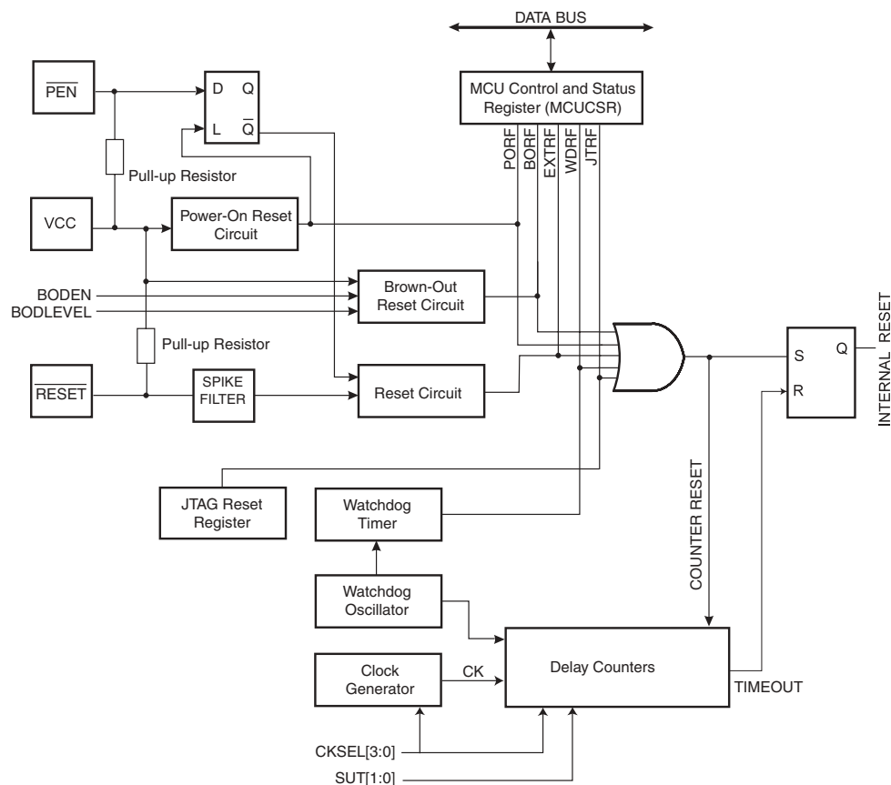
Figure 22. Reset Logic
