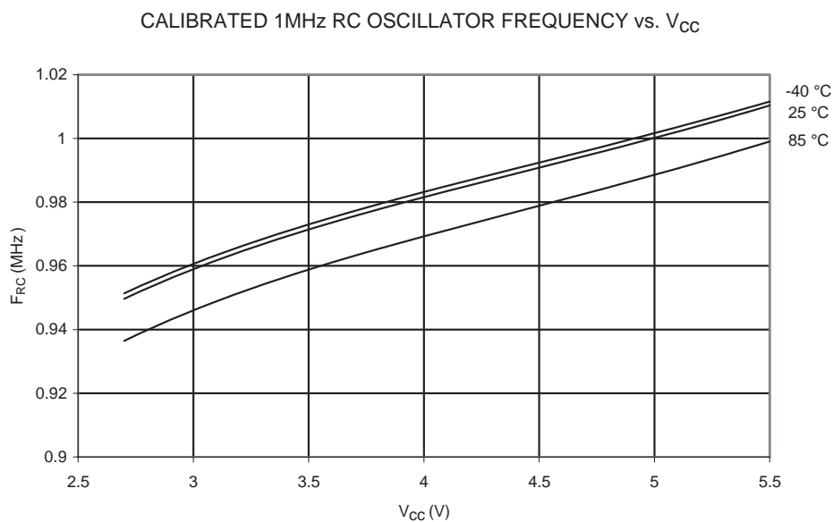
Figure 203. Calibrated 1 MHz RC Oscillator Frequency vs. V_{CC}
