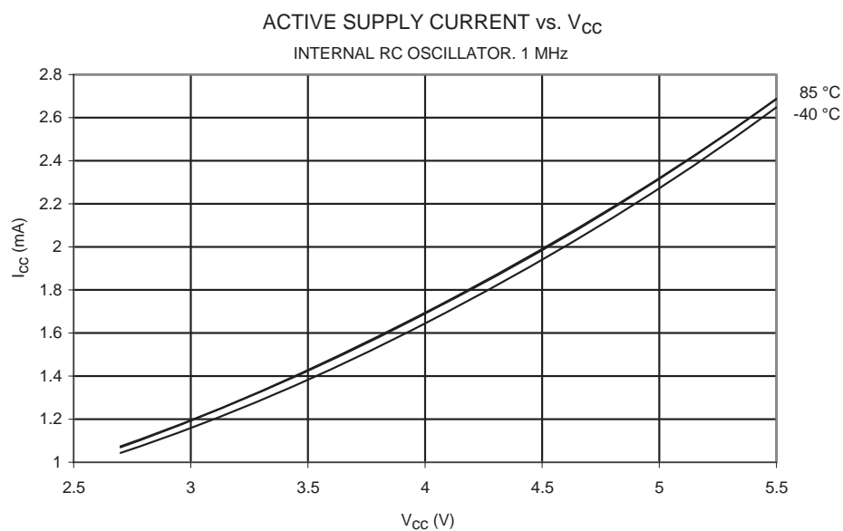
Figure 165. Active Supply Current vs. V_{CC} (Internal RC Oscillator, 1 MHz)
