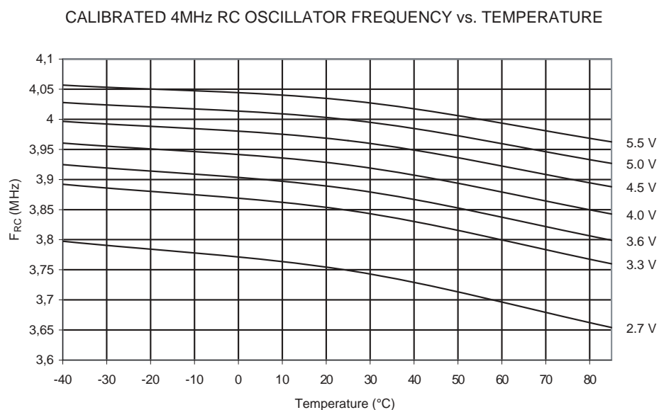
Figure 208. Calibrated 4 MHz RC Oscillator Frequency vs. Temperature
