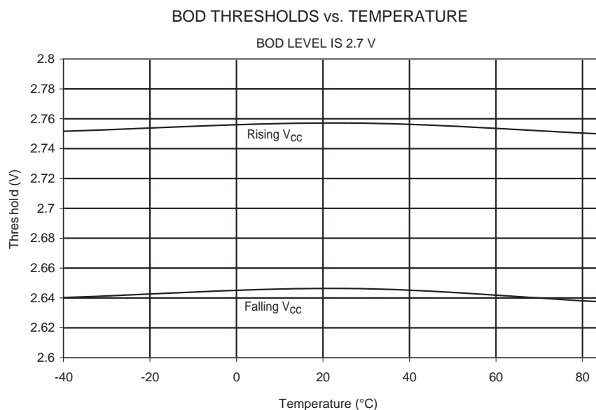
Figure 199. BOD Thresholds vs. Temperature (BODLEVEL is 2.7V)
