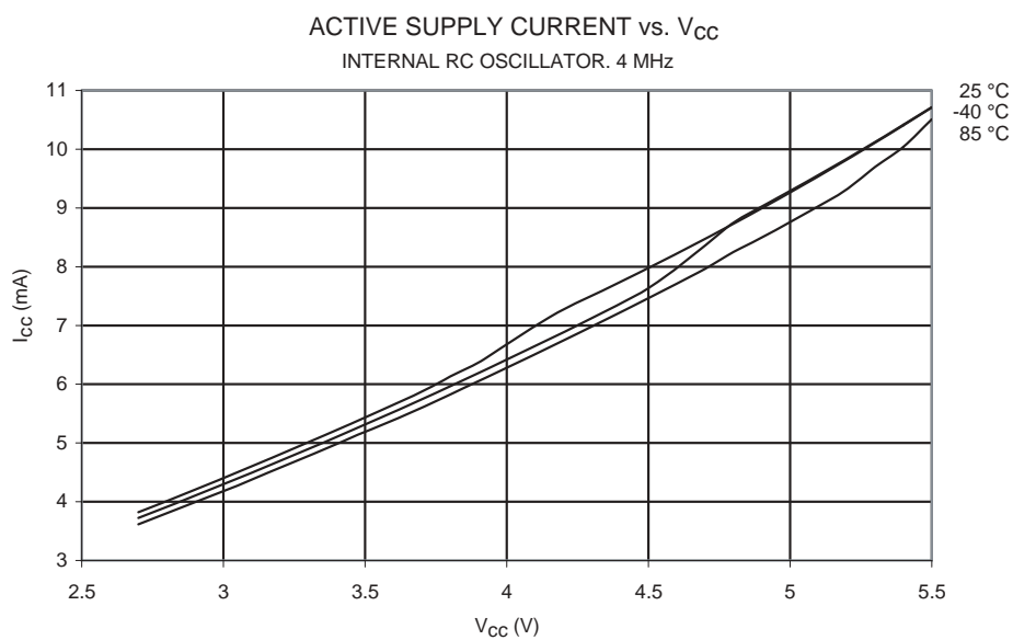
Figure 167. Active Supply Current vs. V_{CC} (Internal RC Oscillator, 4 MHz)
