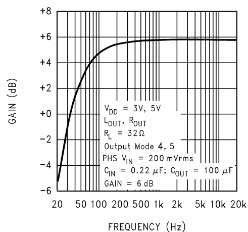
Frequency Response
