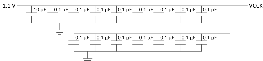
Figure 9-2. VCKK Recommended Filter
