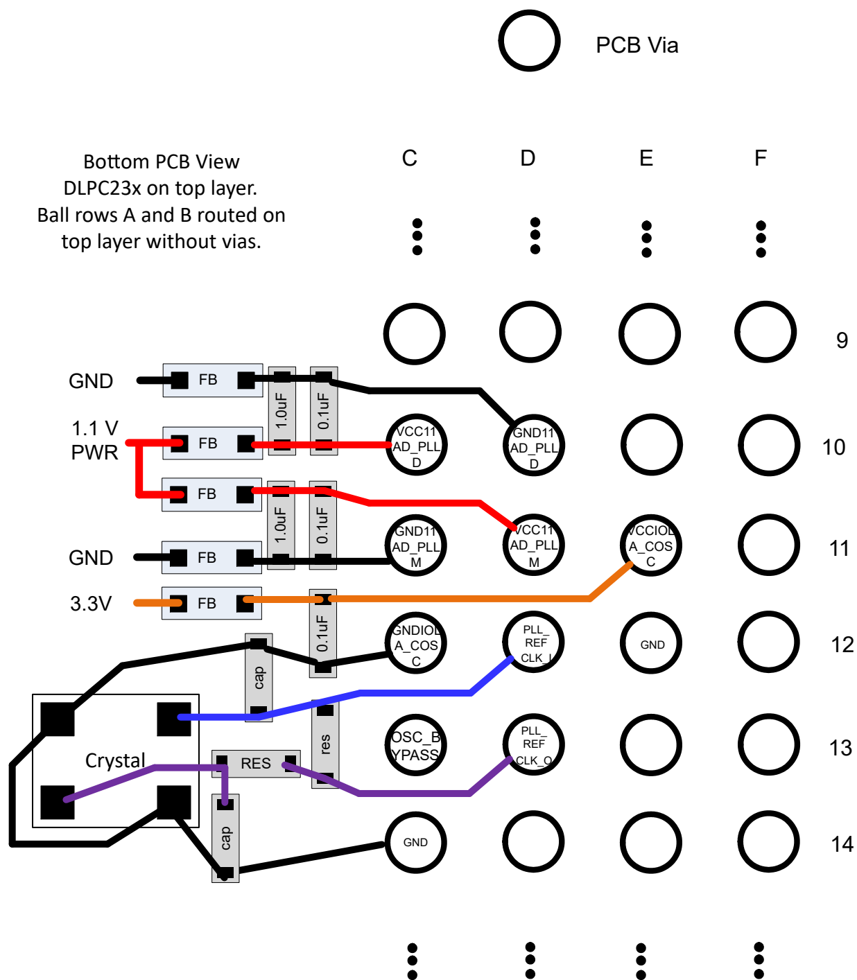
Figure 9-11. DLPC231S-Q1 PLL Filter &amp; Crystal Layout
