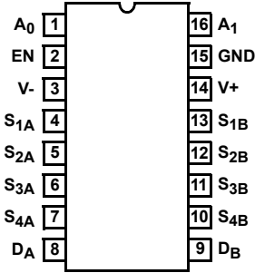
DG409 (PDIP, SOIC, TSSOP) TOP VIEW
