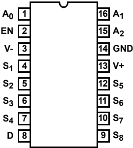
DG408 (PDIP, SOIC, TSSOP) TOP VIEW
