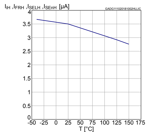
Figure 19. High level logic input current
