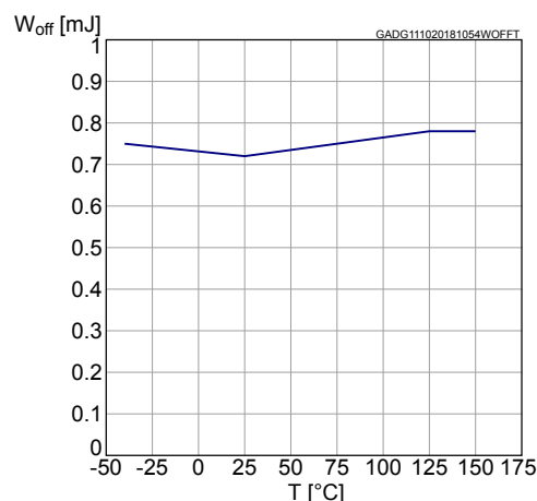
Figure 29. Woff vs. T case
