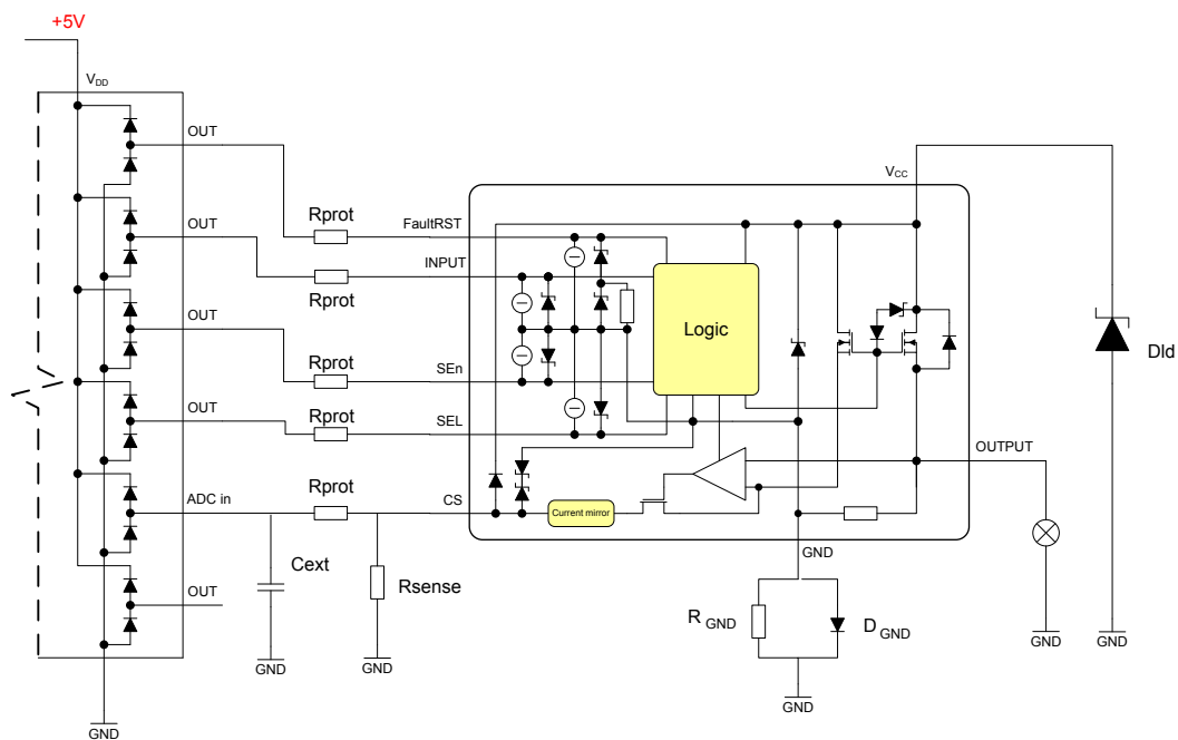
Figure 34. Application diagram
