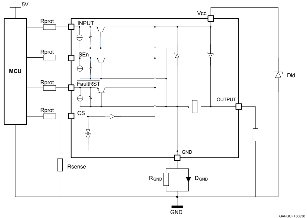
Figure 35. Simplified internal structure
