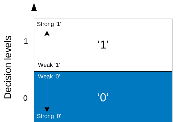
Figure 12-12. Viterbi Hard detection decision levels
