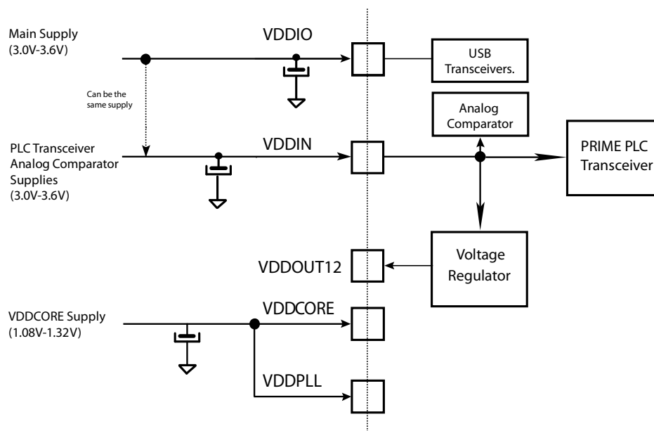
Figure 5-2. Core Externally Supplied
