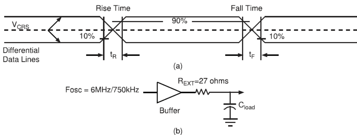
Figure 13-9. USB Data Signal Rise and Fall Times
