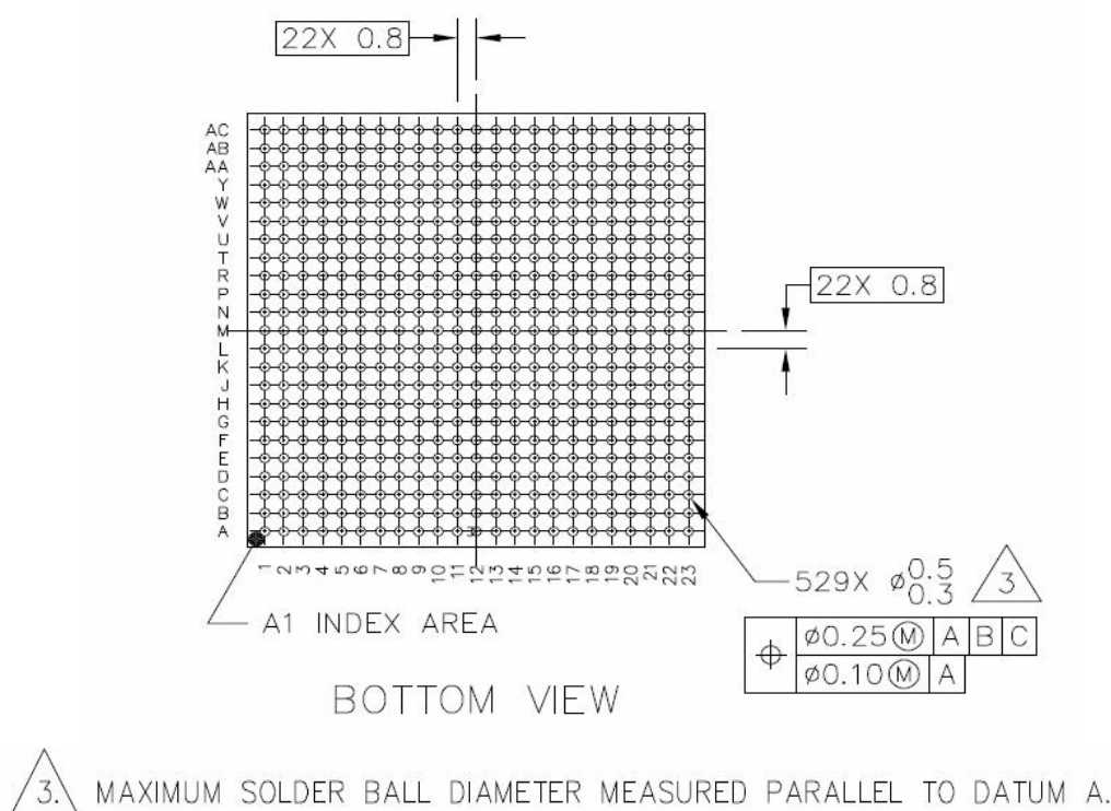
Figure 101. 19 x 19 mm Package, 529 Solder Balls, Bottom View
