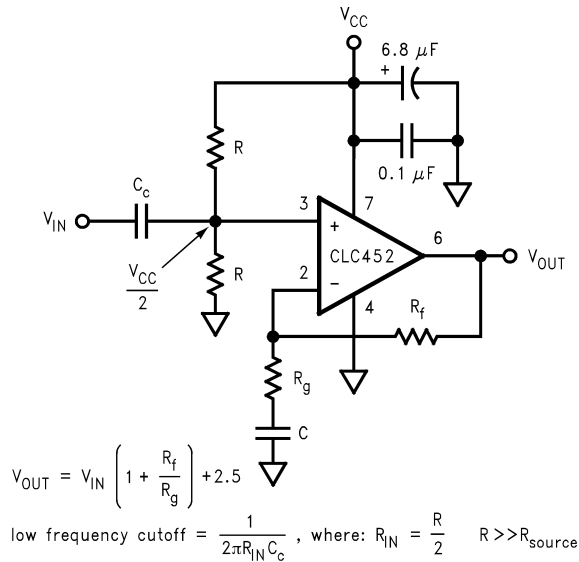
FIGURE 3. AC Coupled Non-Inverting Configuration
