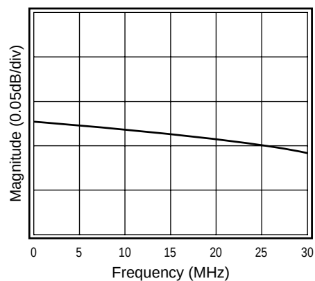
Gain Flatness
