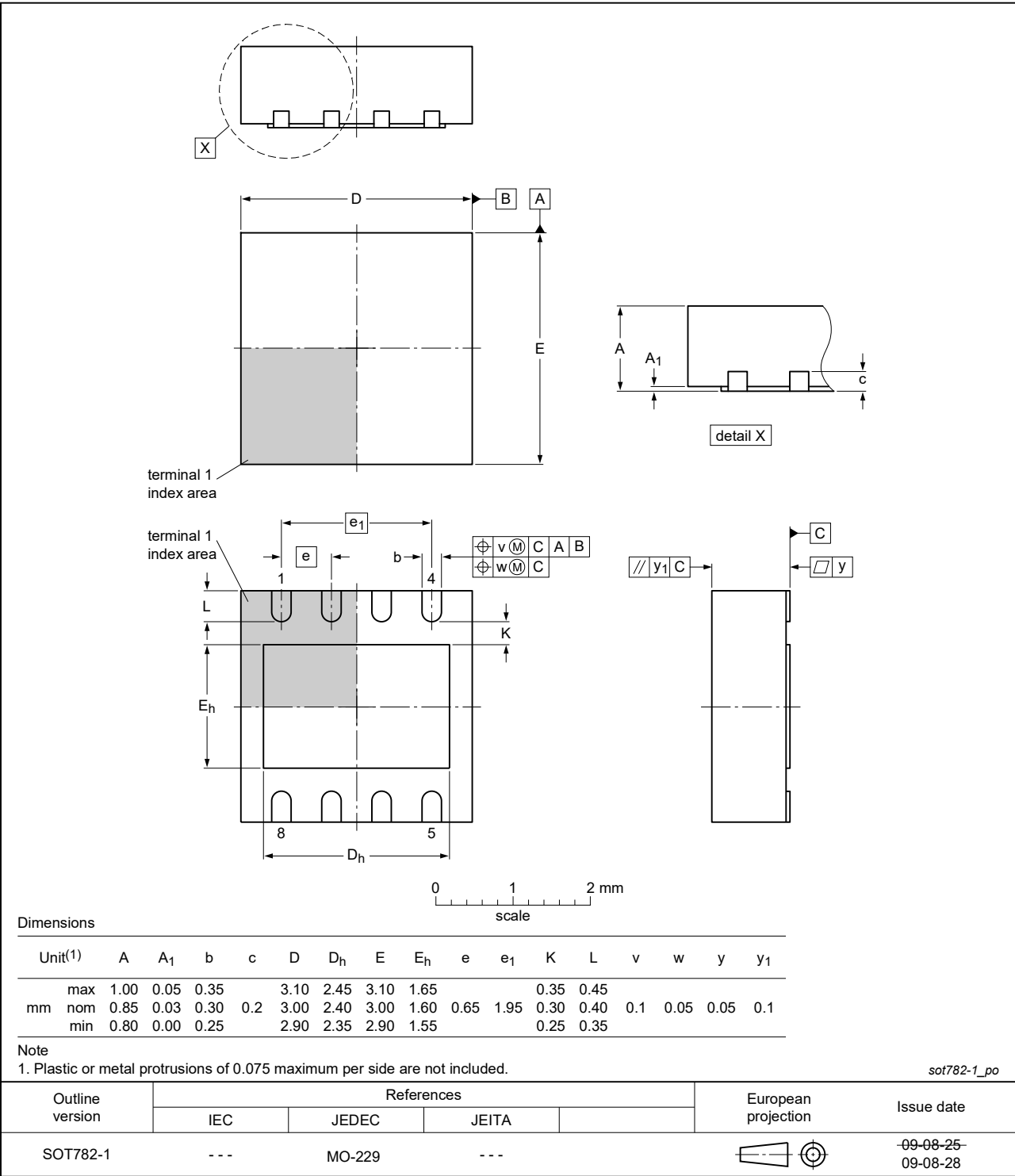
Figure 17. Package outline SOT782-1 (HVSON8)
