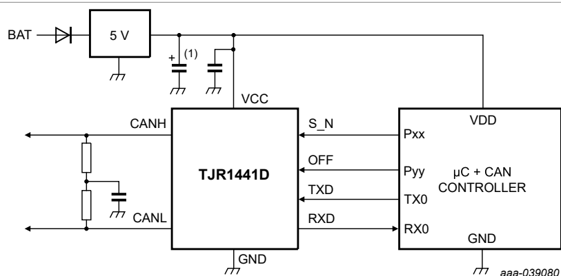
Figure 13. Typical TJR1441D application with a 5 V microcontroller
