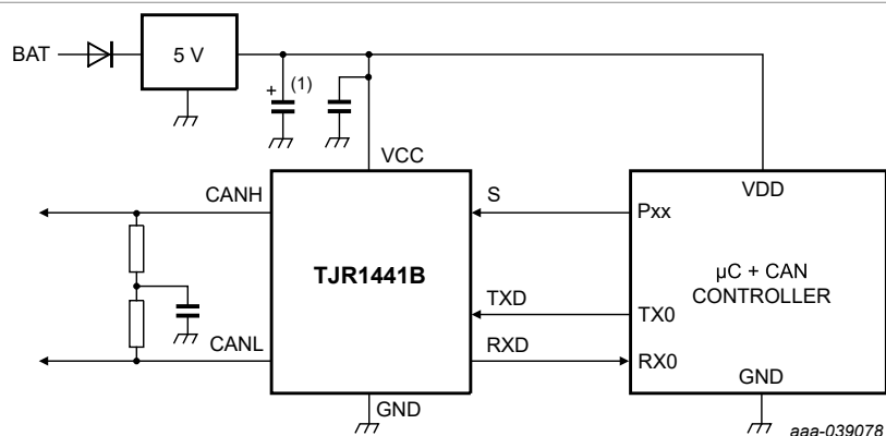
Figure 12. Typical TJR1441B application with a 5 V microcontroller
