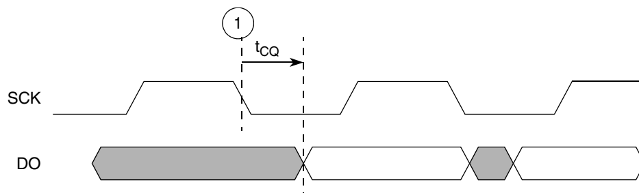
Figure 47. QuadSPI output timing diagram
