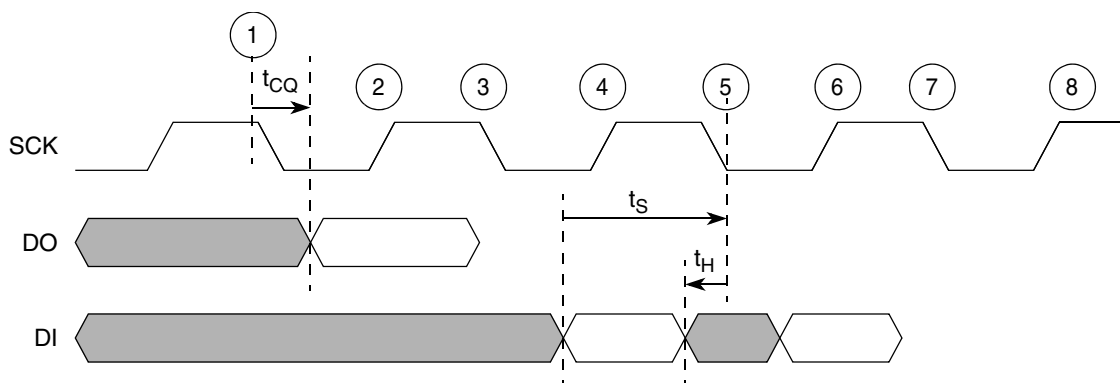
Figure 47. QuadSPI output timing diagram
