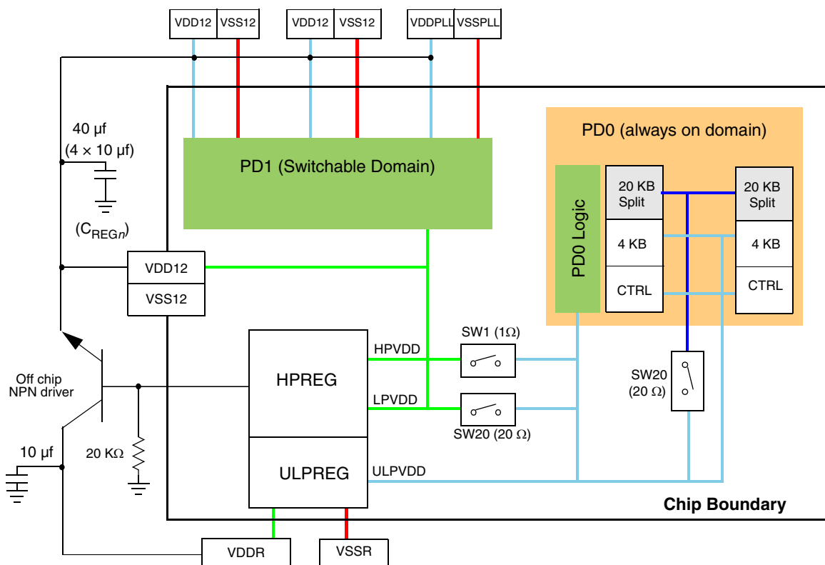
Figure 8. Voltage regulator capacitance connection
