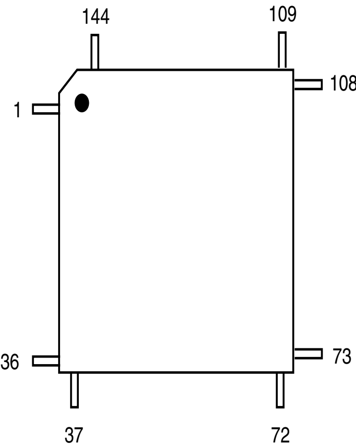
Figure 24-1. 144-lead LQFP Package Orientation (Top View)
