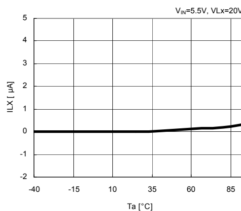
17) Switch Leakage Current vs. Temperature
