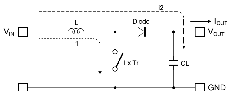
< Typical Circuit >
