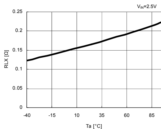
16) Switch ON Resistance vs. Temperature
