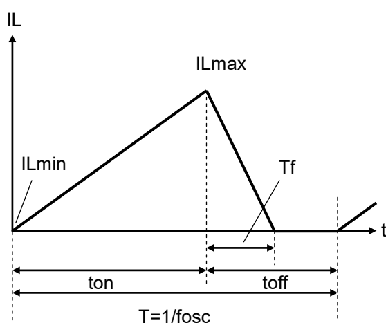
Discontinuous Mode
