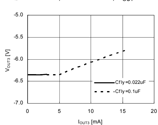
f_{REQ} = 1400\text{kHz} , CPVCC = 8.0\text{V} , V_{OUT} = -6.0\text{V}
