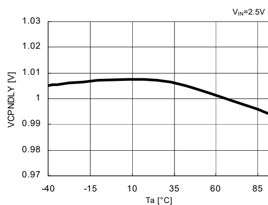
27) CPNDLY Detector Threshold vs. Temperature
