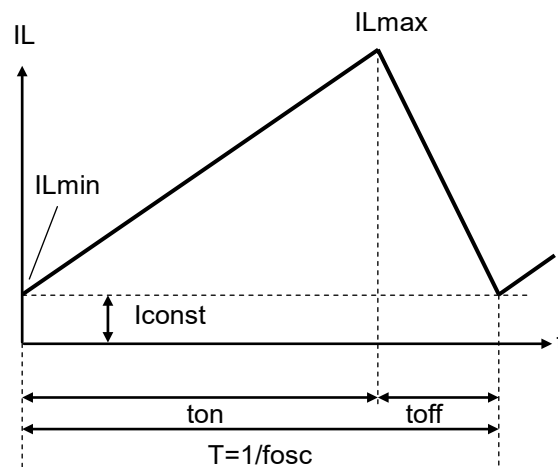
Continuous Mode
