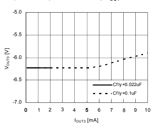
f_{REQ} = 700\text{kHz} , CPVCC = 8.0\text{V} , V_{OUT} = -6.0\text{V}
