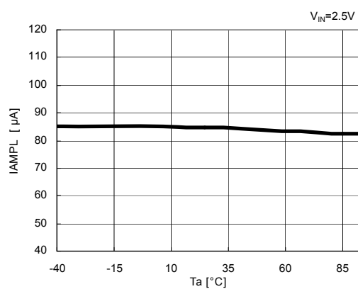
15) AMP"L"Output Current vs. Temperature
