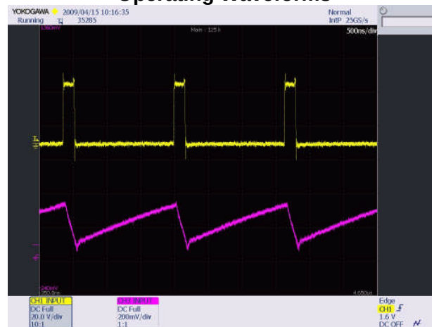
Operating Waveforms
