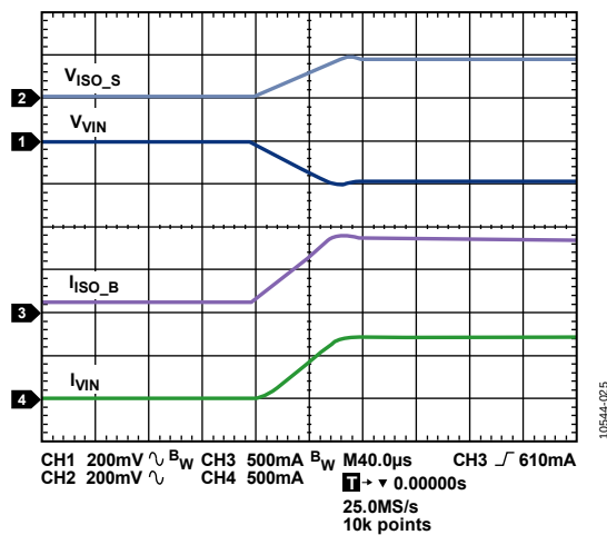
Figure 25. Input Current-Limit Transition from 100 mA to 900 mA, I_{\text{ISO}_S} Load = 66 Ω, Charging = 750 mA
