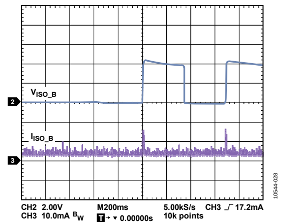
Figure 28. Battery Detection Waveform, \text{VSYSTEM}[2:0] = 000 (Binary) = 4.3 V, No Battery
