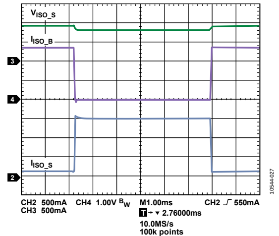
Figure 27. Load Transient. I_{\text{ISO}_S} Load = 300 mA to 1500 mA to 300 mA, \text{EN\_CHG} = \text{High} , \text{ILIM}[3:0] = 0110 (Binary) = 500 mA
