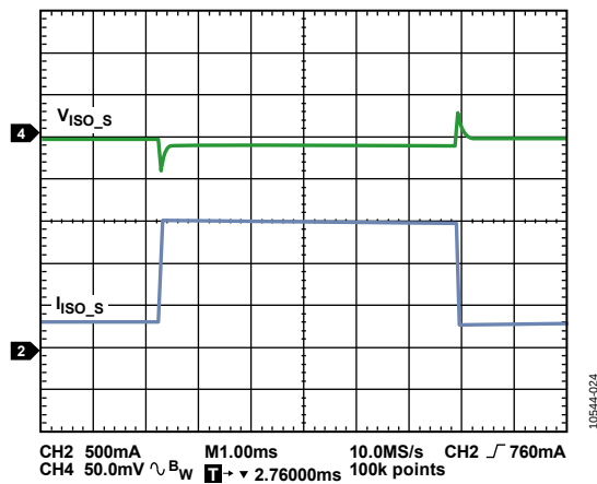
Figure 24. Load Transient, I_{\text{ISO}_S} Load = 300 mA to 1500 mA to 300 mA
