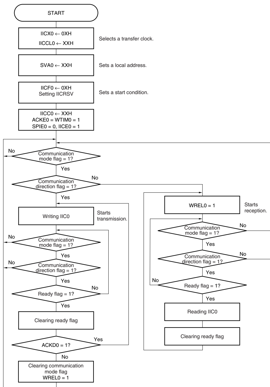
★ Figure 17-25. Slave Operation Flowchart (1)
