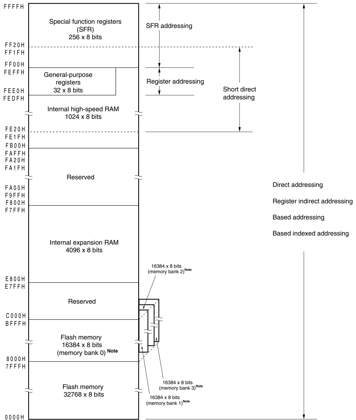
Figure 3-14. Correspondence Between Data Memory and Addressing ( \mu PD78F0536)
