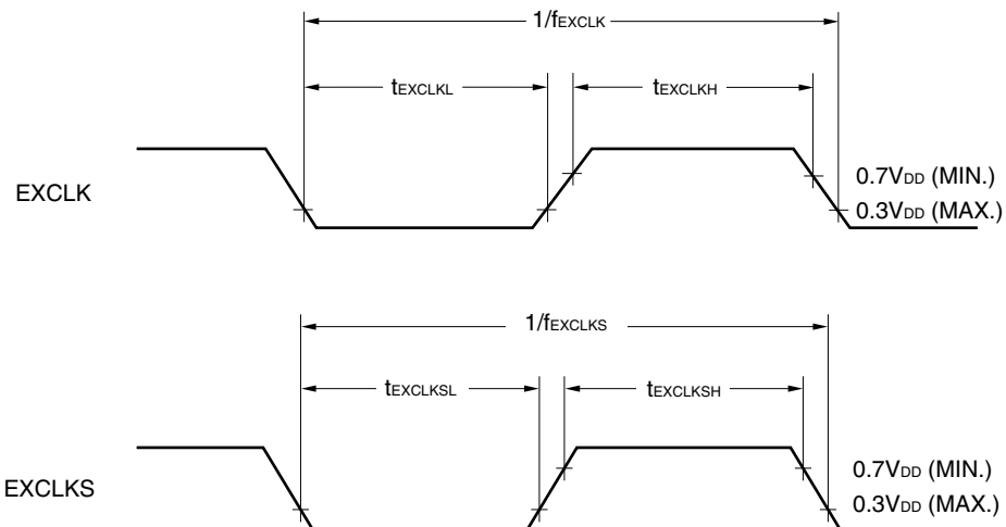
External Main System Clock Timing, External Subsystem Clock Timing
