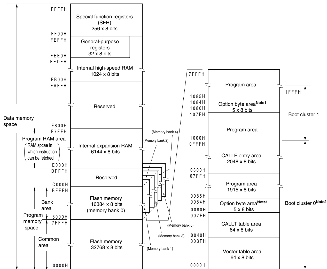
Figure 3-7. Memory Map (μPD78F0537)
