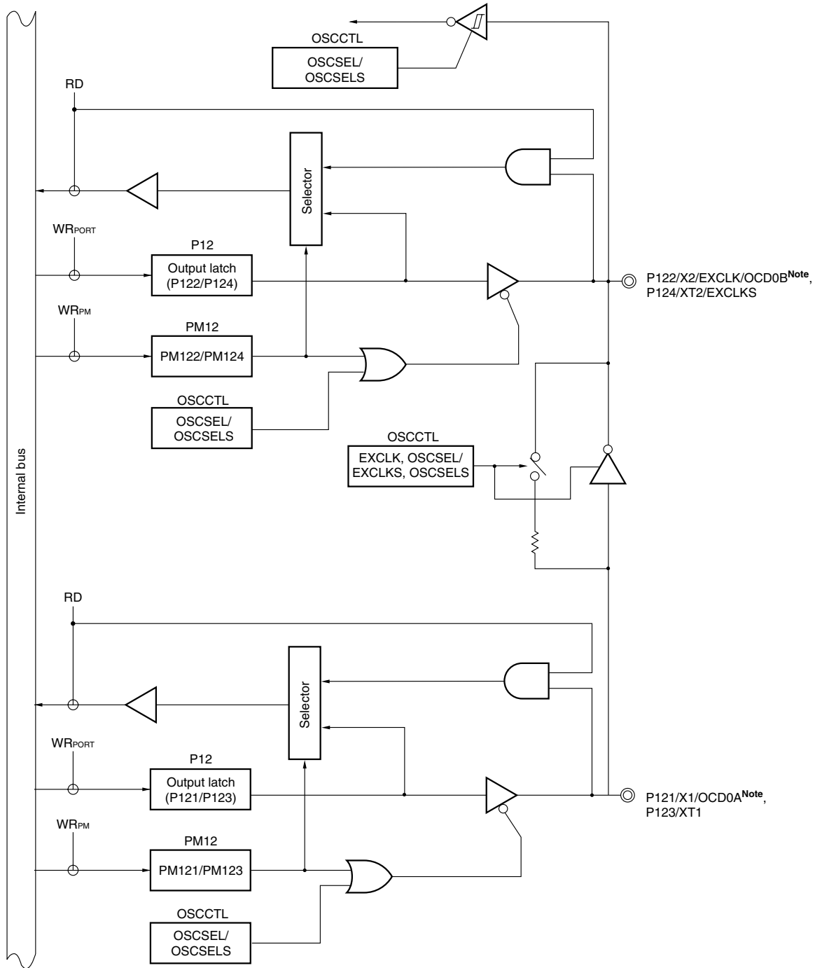
Figure 5-23. Block Diagram of P121 to P124
