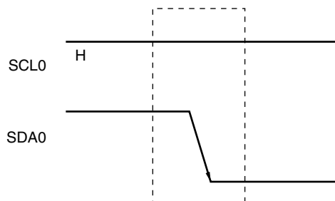
Figure 17-13. Start Conditions
