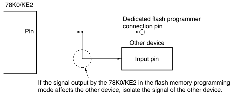
Figure 26-10. Malfunction of Other Device
