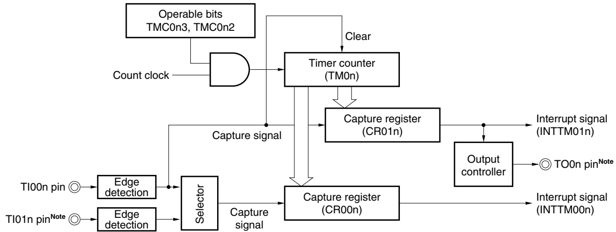
Figure 7-33. Block Diagram of Clear & Start Mode Entered by TI00n Pin Valid Edge Input (CR00n: Capture Register, CR01n: Capture Register)
