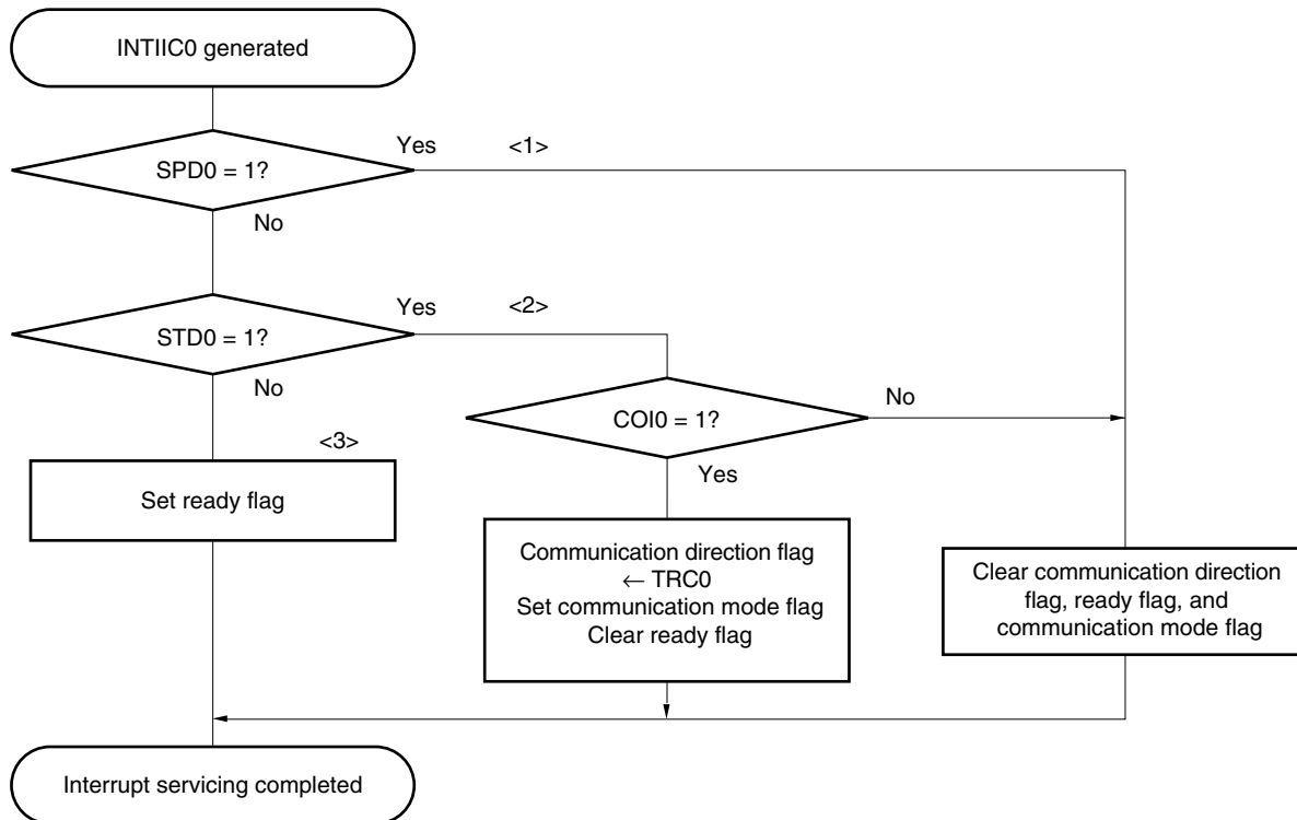
Figure 17-26. Slave Operation Flowchart (2)
