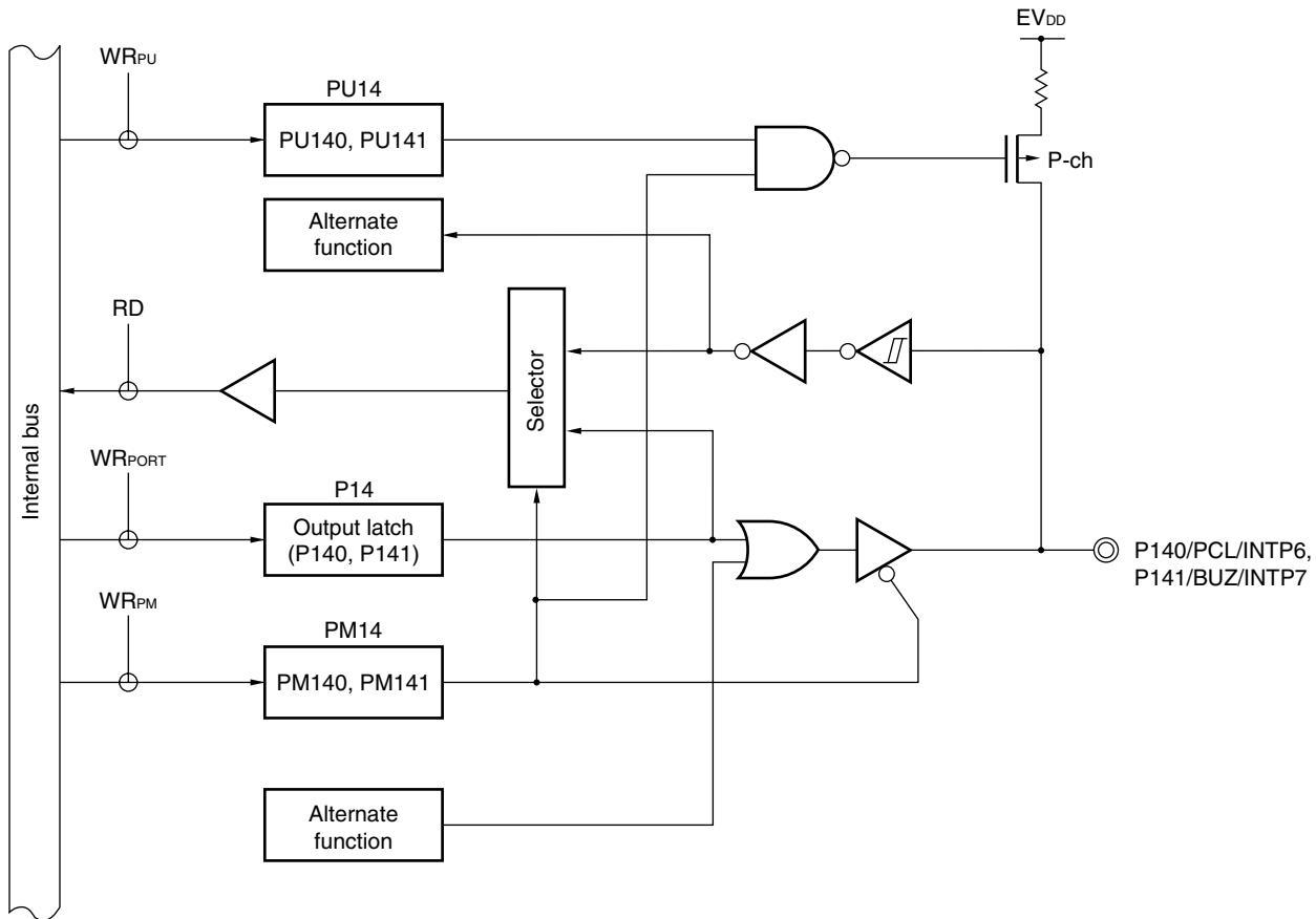
Figure 5-25. Block Diagram of P140 and P141
