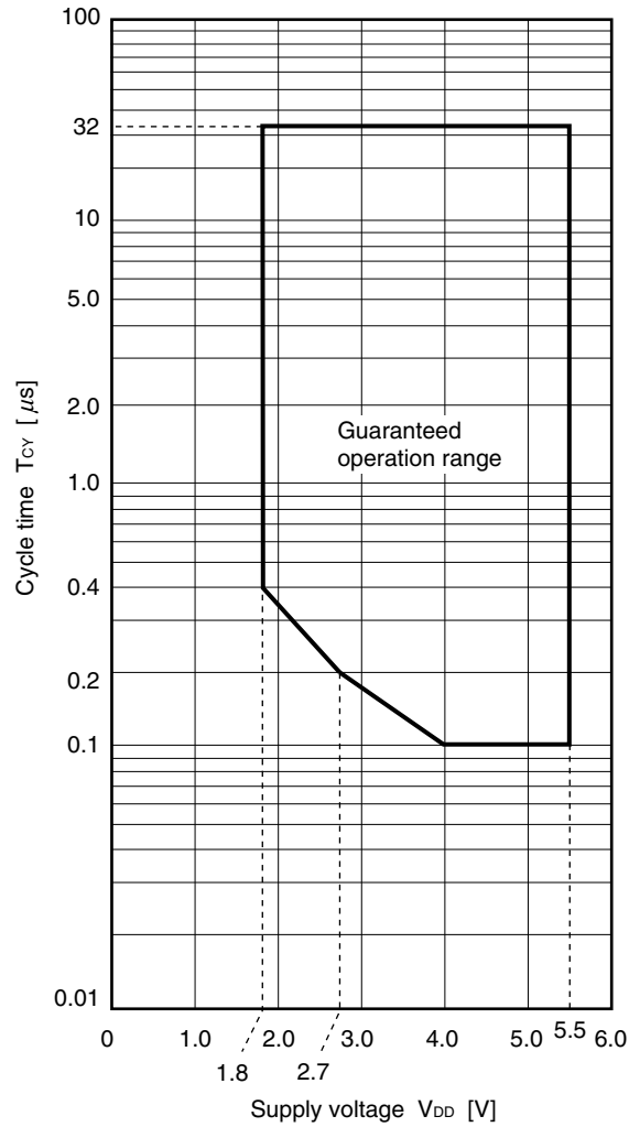
AC Timing Test Points (Excluding External Main System Clock and External Subsystem Clock)
