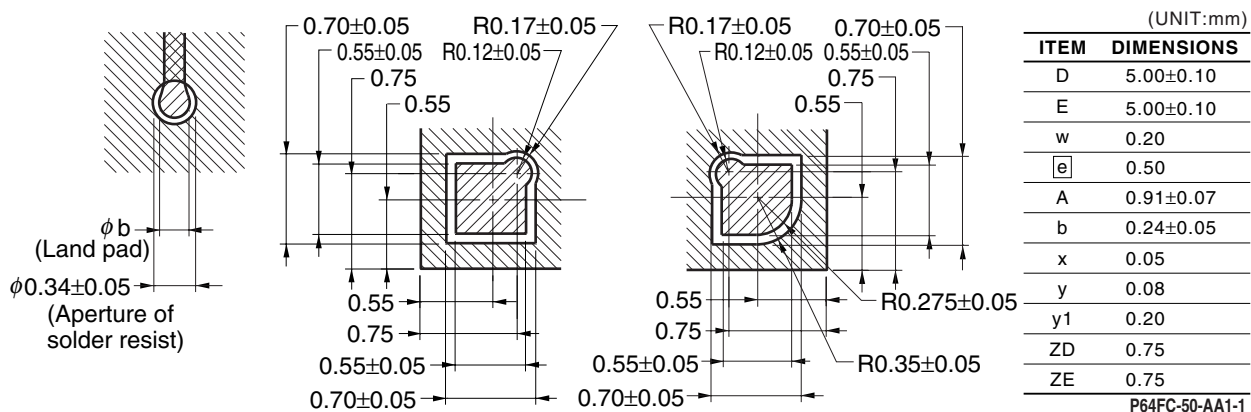
DETAIL OF (C) PART
