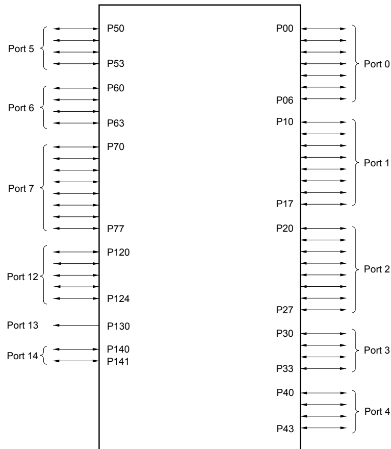
Figure 5-1. Port Types
