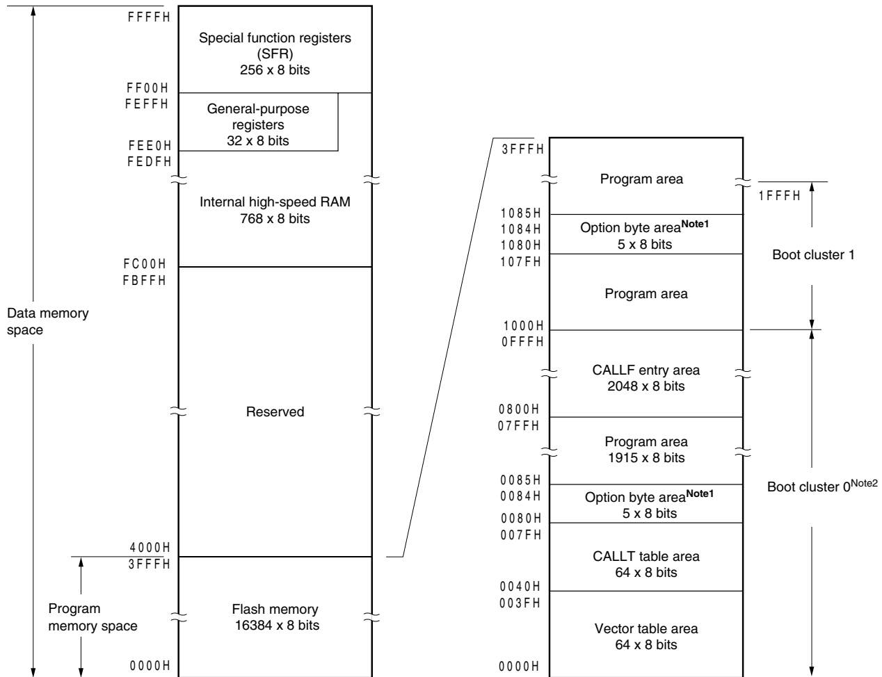
Figure 3-1. Memory Map (μPD78F0531)
