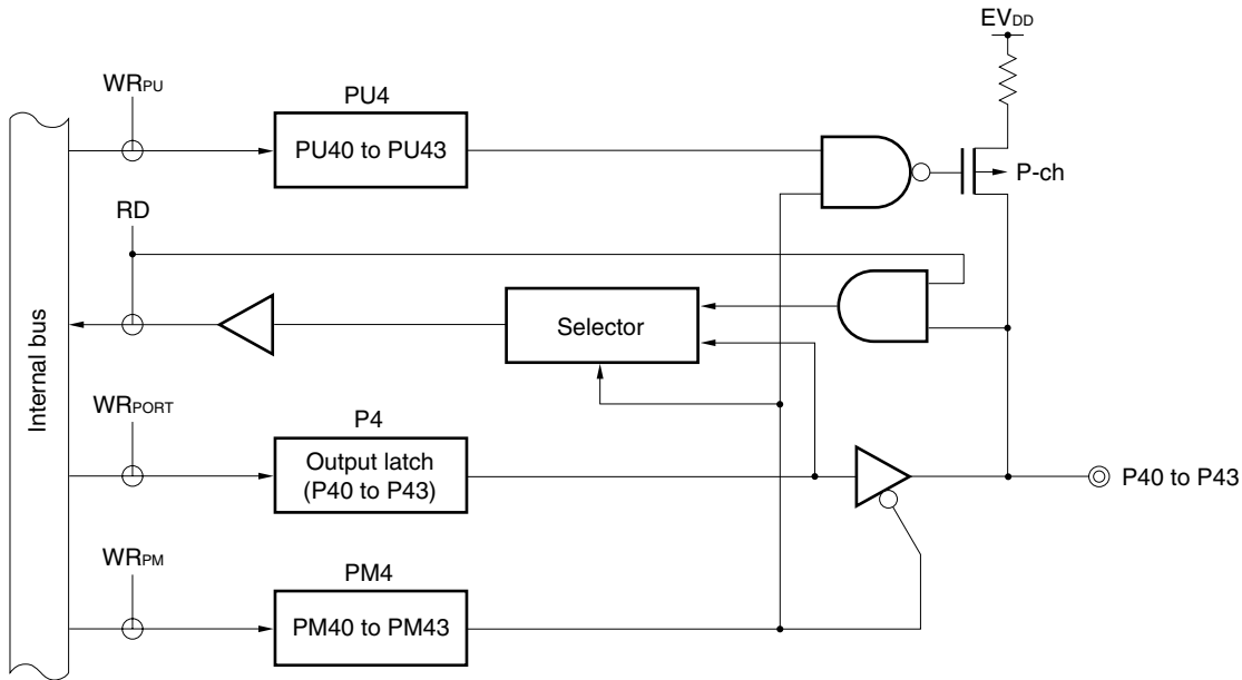
Figure 5-16. Block Diagram of P40 to P43
