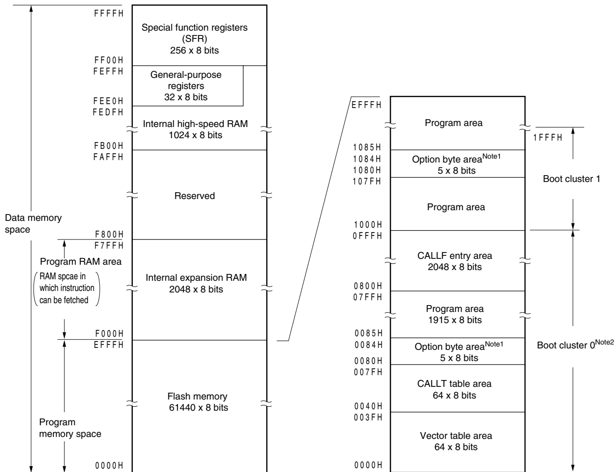
Figure 3-5. Memory Map (μPD78F0535)
