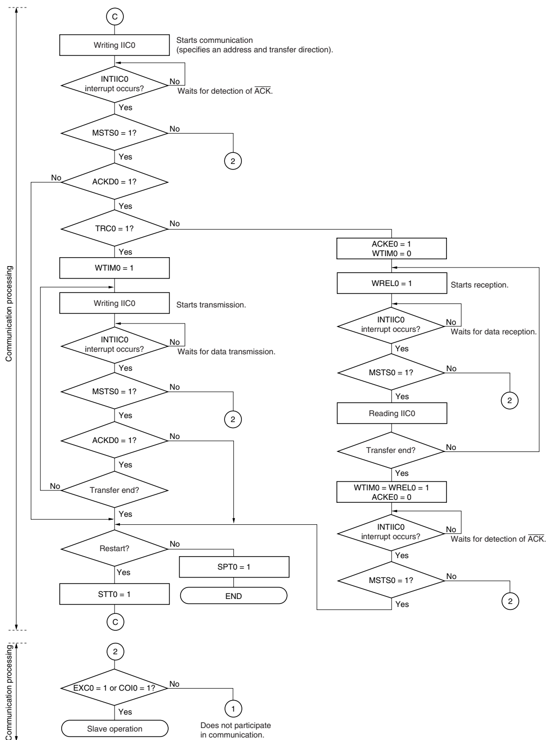
Figure 17-24. Master Operation Flowchart (Multi-Master System) (3/3)
