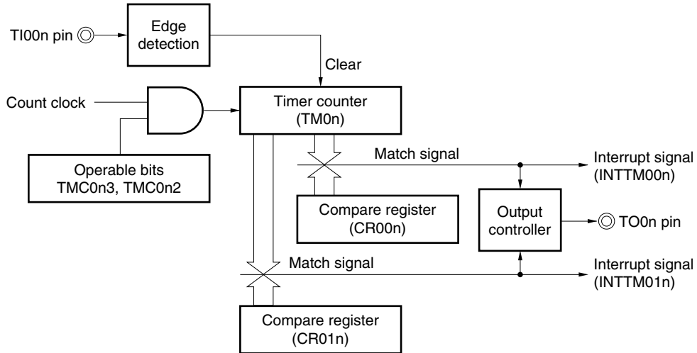
Figure 7-27. Block Diagram of Clear & Start Mode Entered by TI00n Pin Valid Edge Input (CR00n: Compare Register, CR01n: Compare Register)
