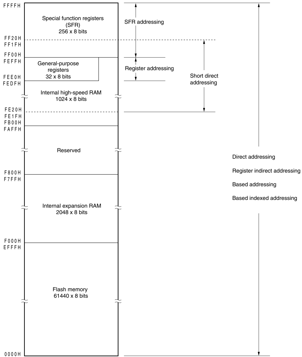
Figure 3-13. Correspondence Between Data Memory and Addressing ( \mu PD78F0535)
