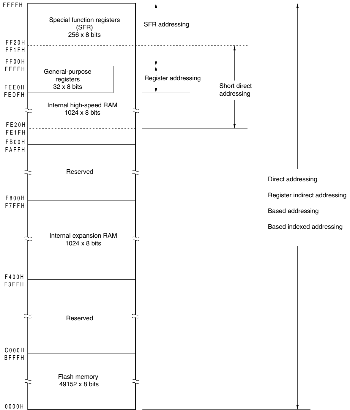
Figure 3-12. Correspondence Between Data Memory and Addressing ( \mu PD78F0534)
