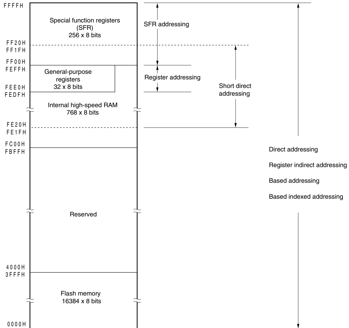
Figure 3-9. Correspondence Between Data Memory and Addressing ( \mu PD78F0531)
