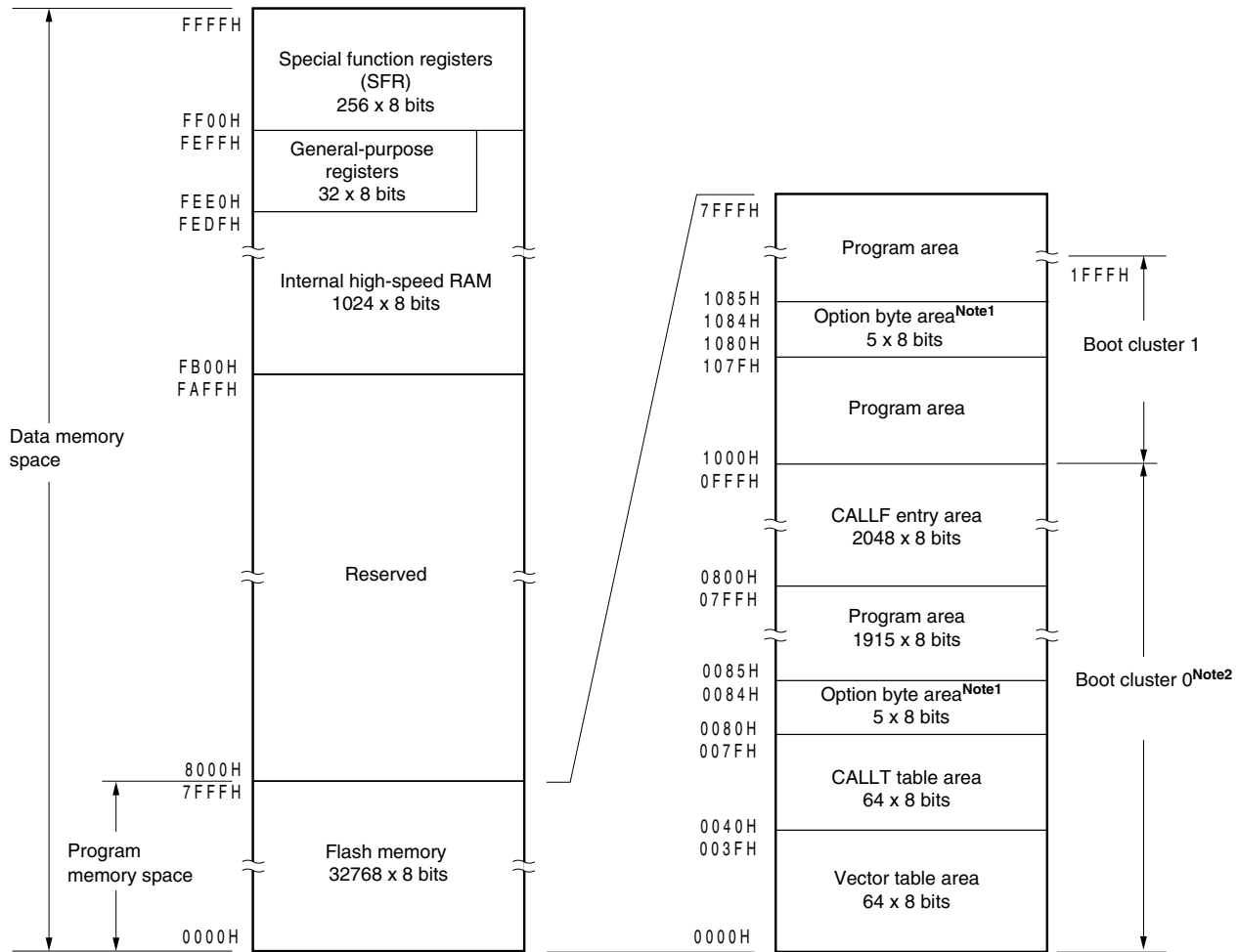
Figure 3-3. Memory Map (μPD78F0533)
