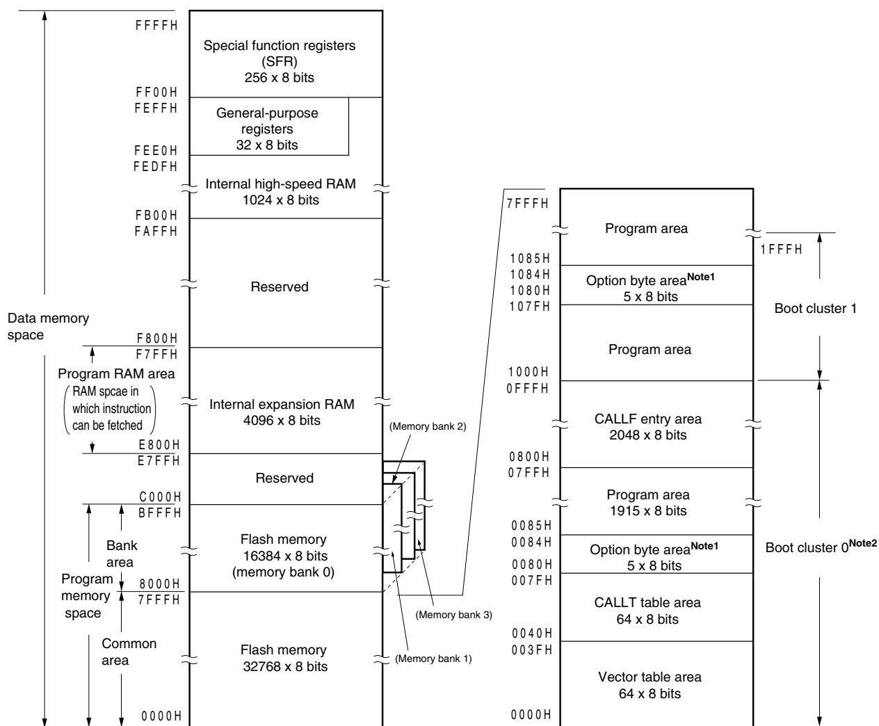
Figure 3-6. Memory Map (μPD78F0536)
