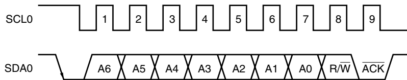
Figure 17-16. \overline{\text{ACK}}
