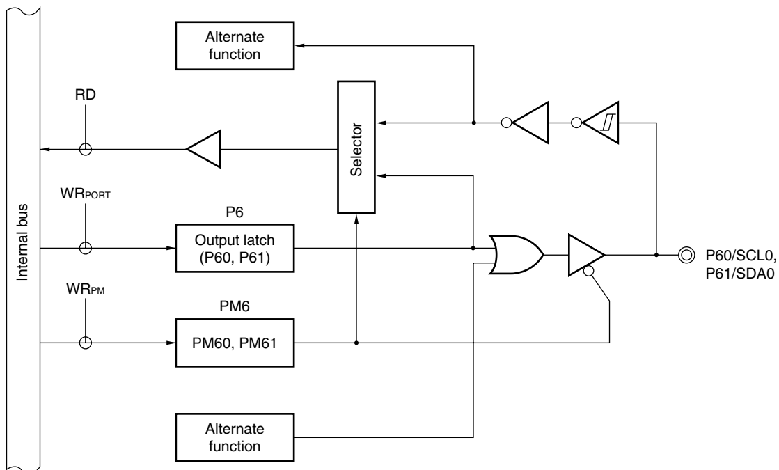
Figure 5-18. Block Diagram of P60 and P61
