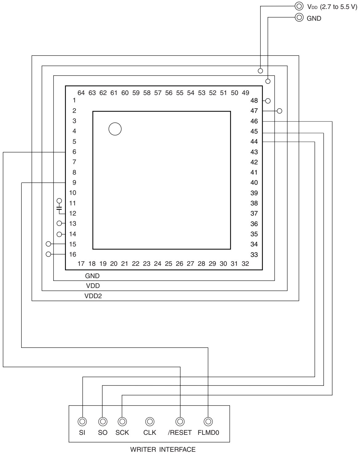
★ Figure 26-3. Example of Wiring Adapter for Flash Memory Writing in 3-Wire Serial I/O (CSI10) Mode
