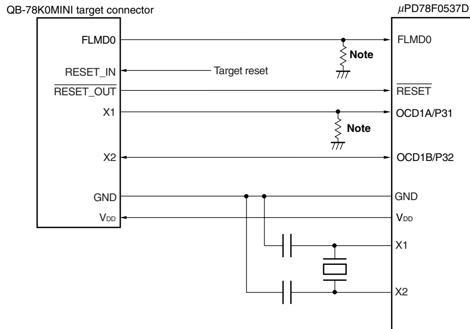
Figure 27-2. Connection Example of QB-78K0MINI and \mu PD78F0537D (When OCD1A and OCD1B Are Used)
