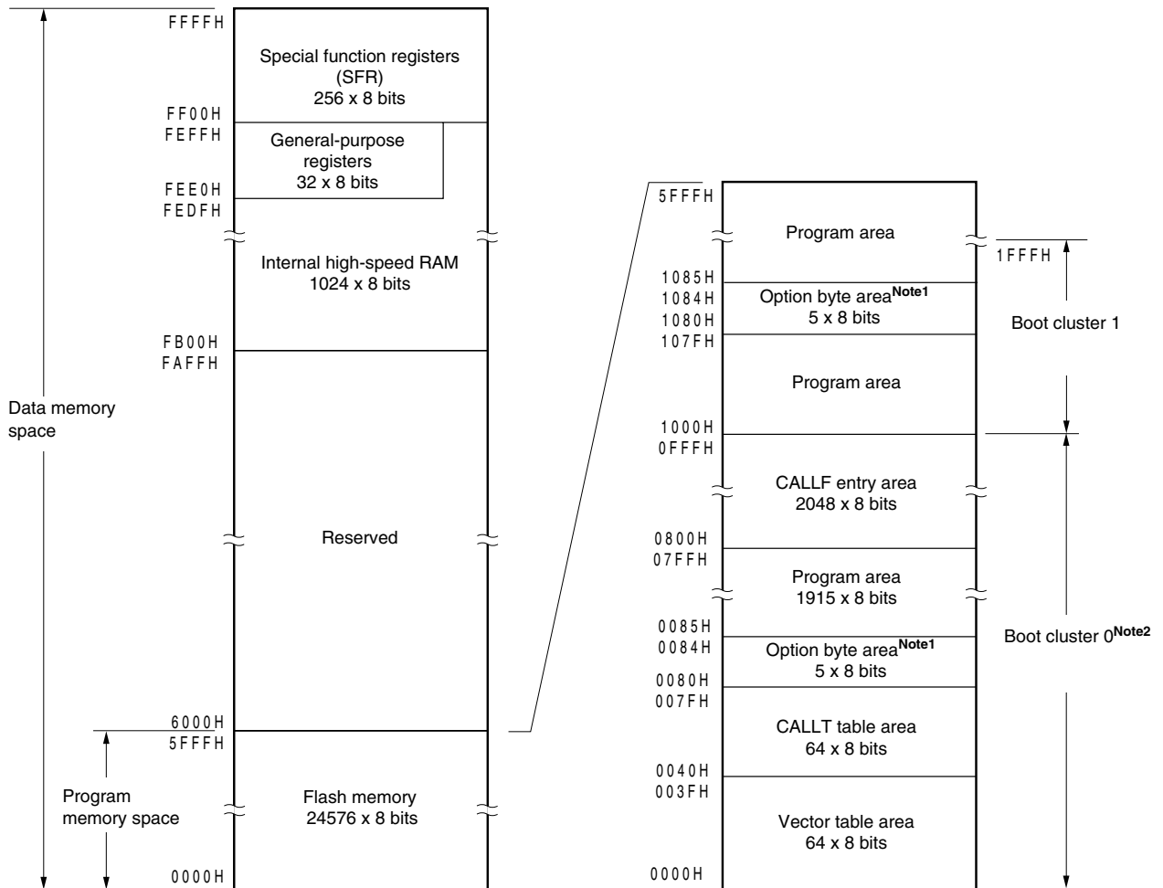
Figure 3-2. Memory Map ( \mu PD78F0532)
