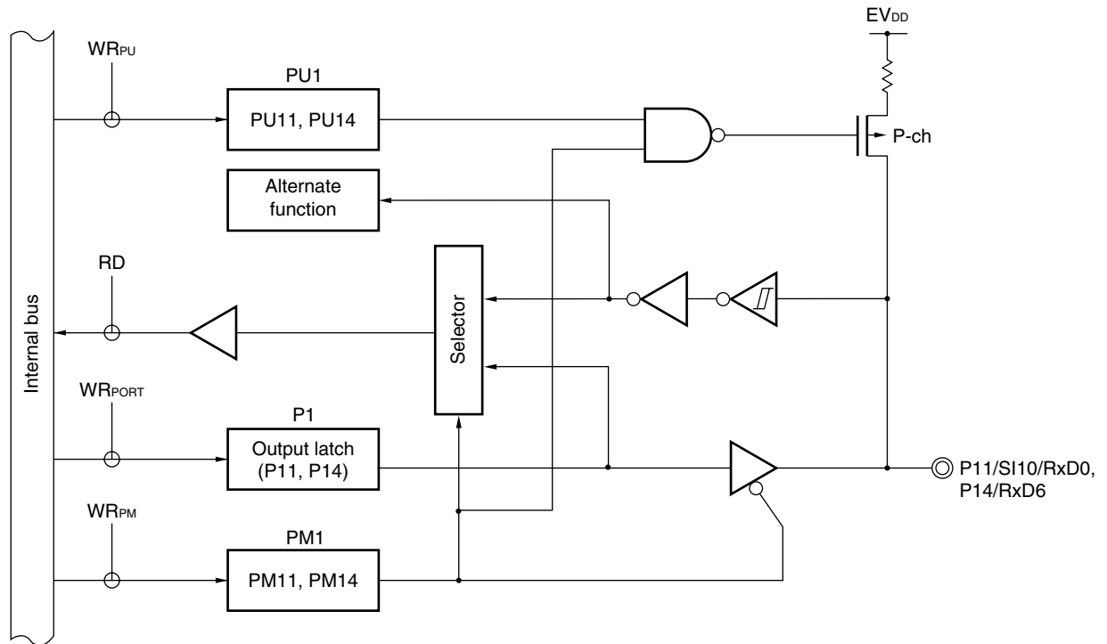
Figure 5-9. Block Diagram of P11 and P14
