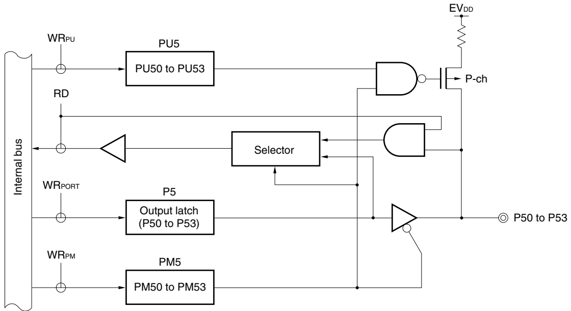
Figure 5-17. Block Diagram of P50 to P53
