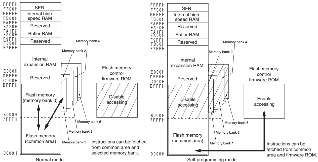
Figure 26-15. Operation Mode and Memory Map for Self-Programming ( \mu PD78F0537)
