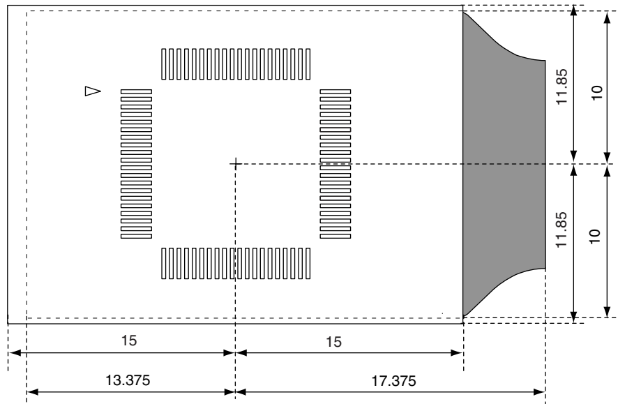
Figure B-2. For 64-Pin GC Package
