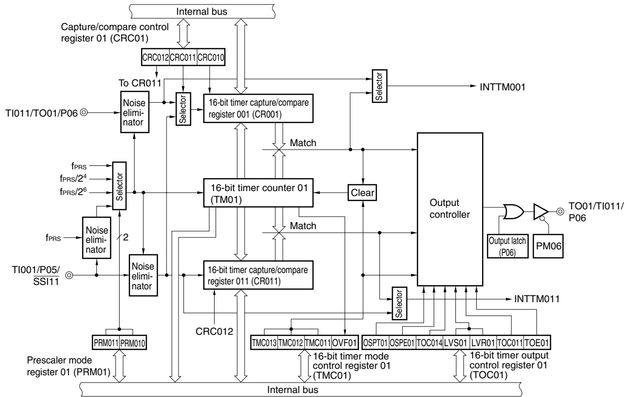
Figure 7-2. Block Diagram of 16-Bit Timer/Event Counter 01 (Available only in the \mu PD78F0534, 78F0535, 78F0536, 78F0537, and 78F0537D)
