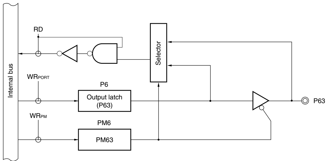
Figure 5-20. Block Diagram of P63
