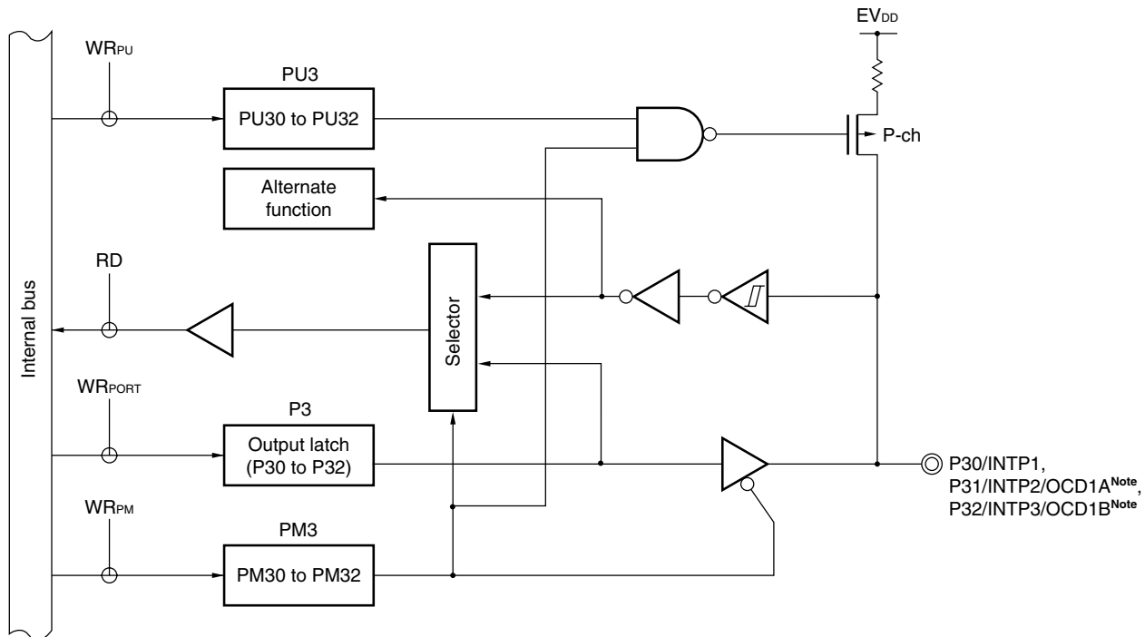
Figure 5-14. Block Diagram of P30 to P32
