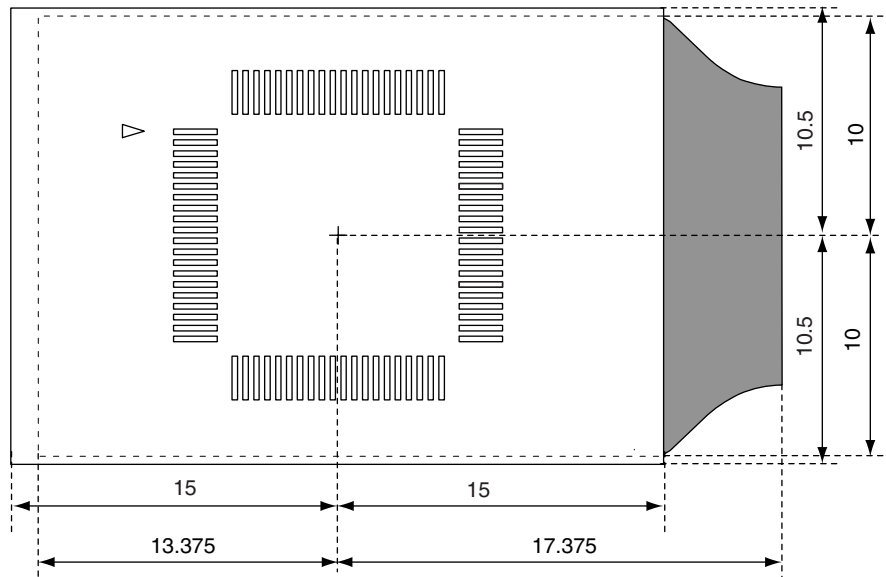
Figure B-3. For 64-Pin GK Package
