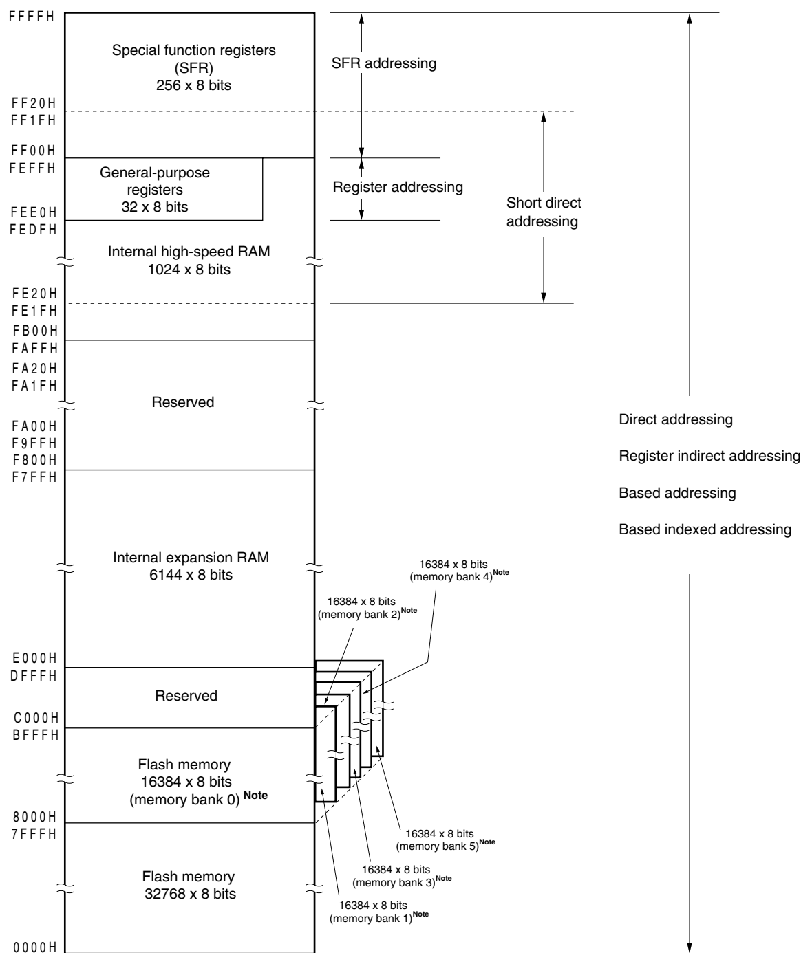
Figure 3-15. Correspondence Between Data Memory and Addressing ( \mu PD78F0537, 78F0537D)
