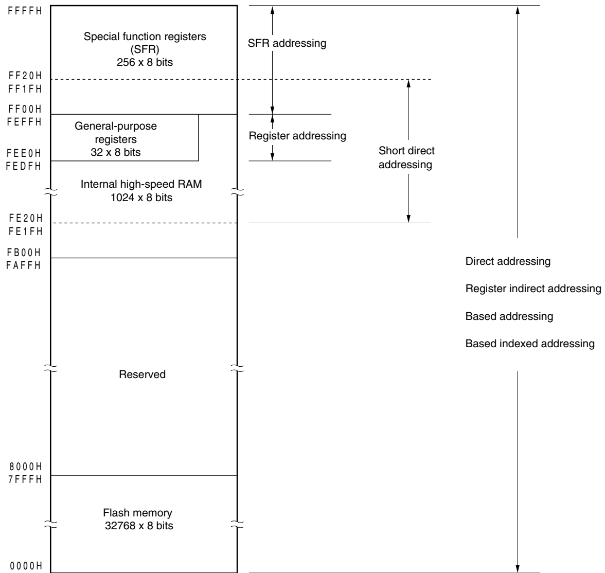
Figure 3-11. Correspondence Between Data Memory and Addressing ( \mu PD78F0533)
