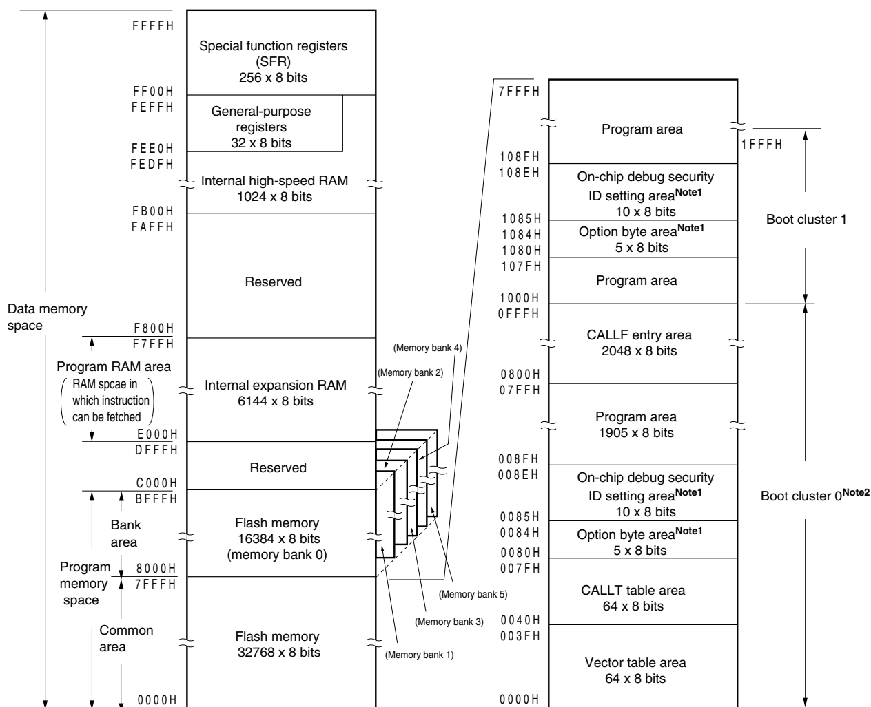
Figure 3-8. Memory Map ( \mu PD78F0537D)
