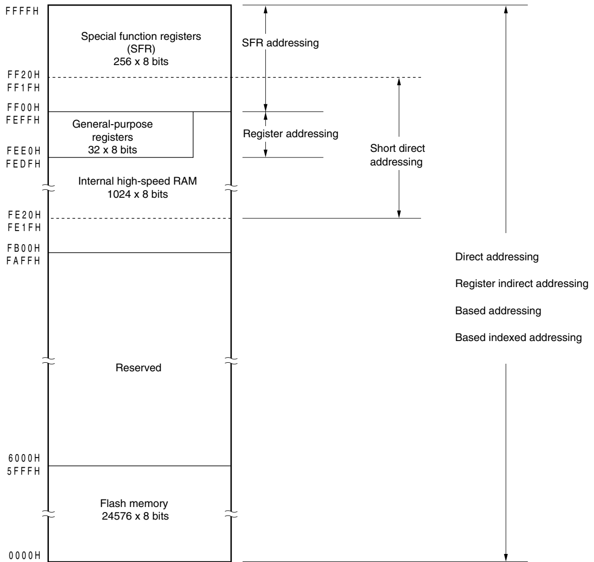
Figure 3-10. Correspondence Between Data Memory and Addressing ( \mu PD78F0532)
