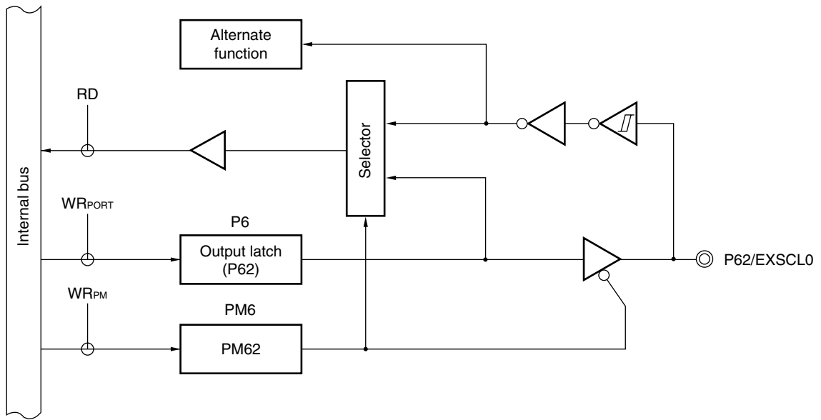
Figure 5-19. Block Diagram of P62
