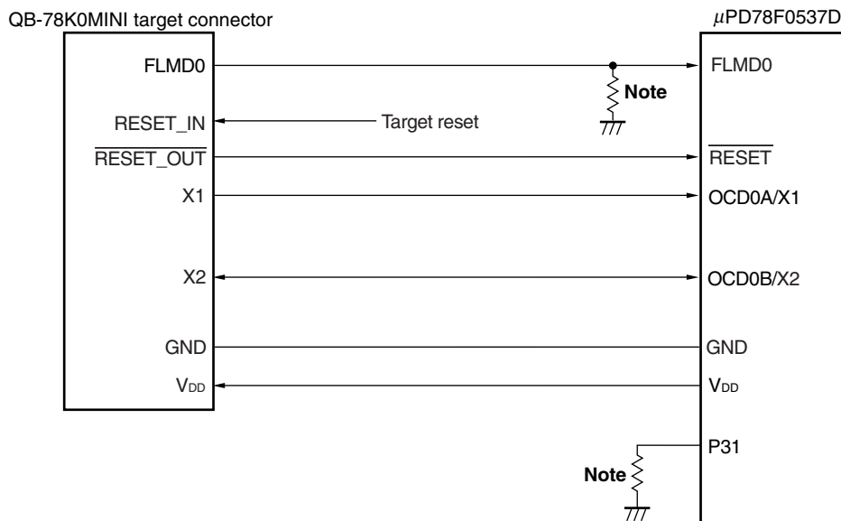
Figure 27-1. Connection Example of QB-78K0MINI and \mu PD78F0537D (When OCD0A/X1 and OCD0B/X2 Are Used)
