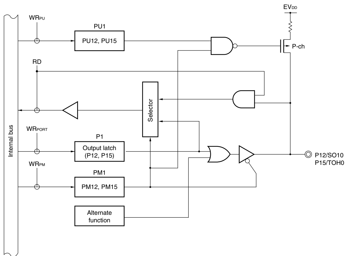
Figure 5-10. Block Diagram of P12 and P15
