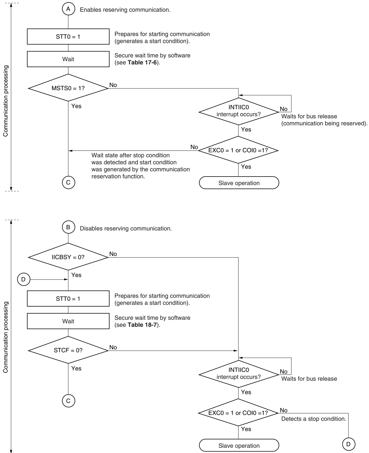
Figure 17-24. Master Operation Flowchart (Multi-Master System) (2/3)
