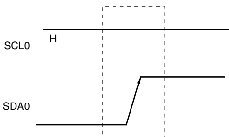
Figure 17-17. Stop Condition
