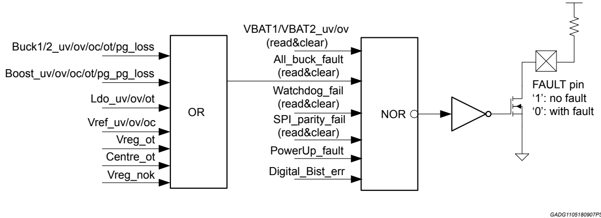
Figure 14. Fault function in active mode
