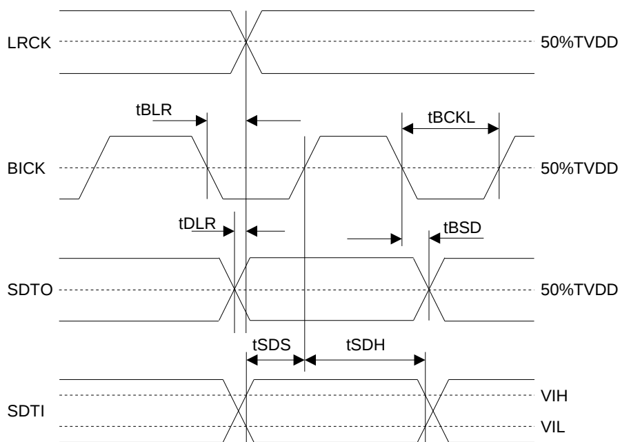
Figure 6. Audio Interface Timing (PLL/EXT Master mode)
