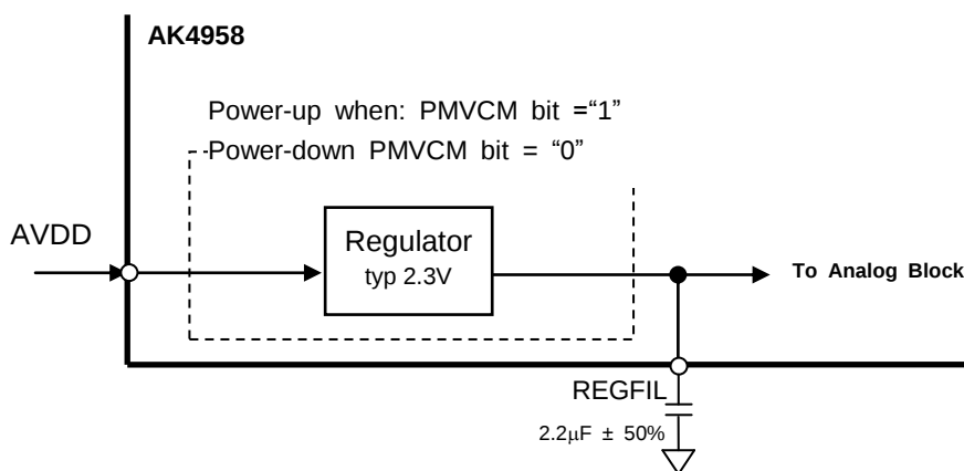
Figure 68 Regulator Block
