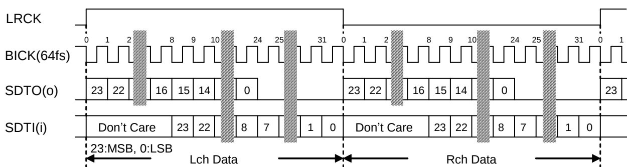
Figure 27. Mode 0 Timing
