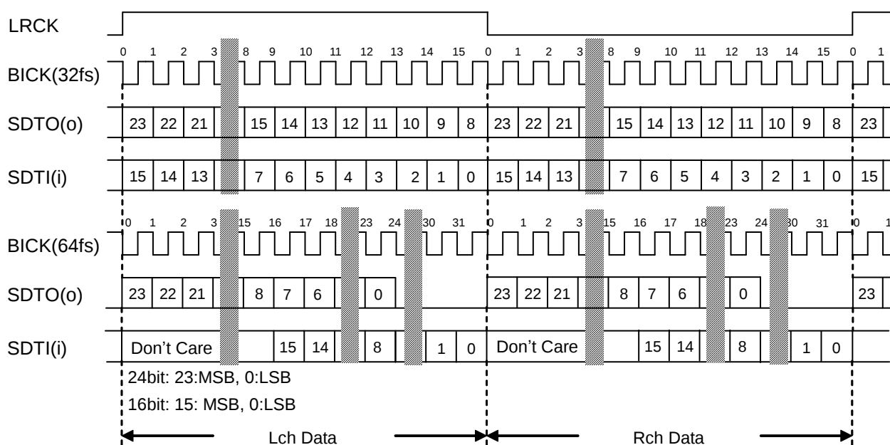
Figure 28. Mode 1 Timing
