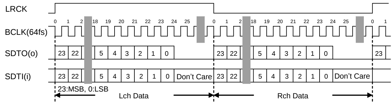
Figure 29. Mode 2 Timing
