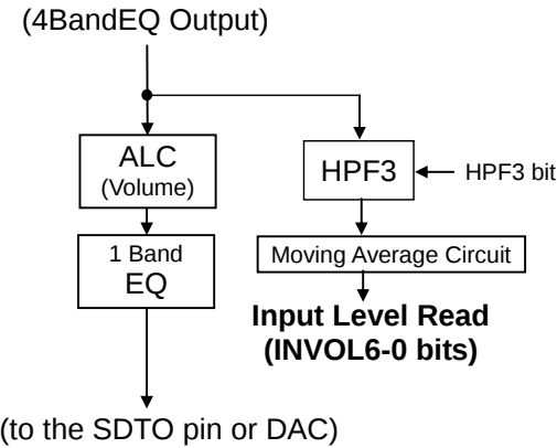
Figure 46. ALC Input Level Read Function
