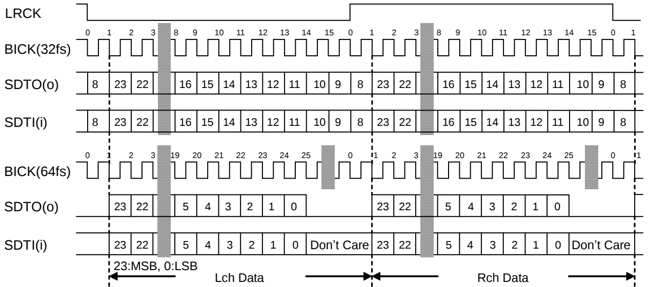
Figure 30. Mode 3 Timing
