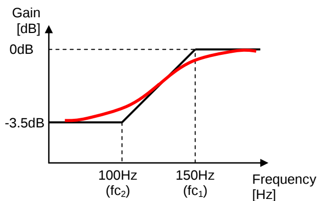
Figure 48. ALCEQ Frequency Response ( f_s = 48\text{kHz} )
