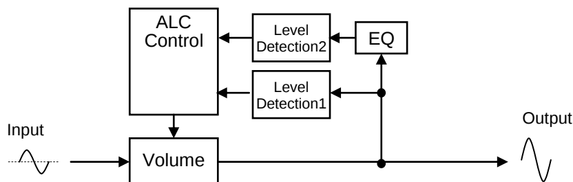
Figure 47. ALC Block
