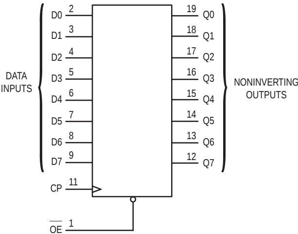
LOGIC DIAGRAM
