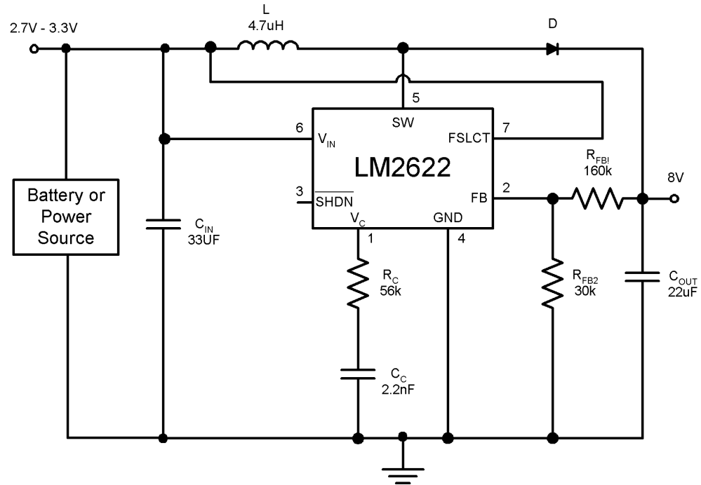
FIGURE 5. 1.3 MHz operation
