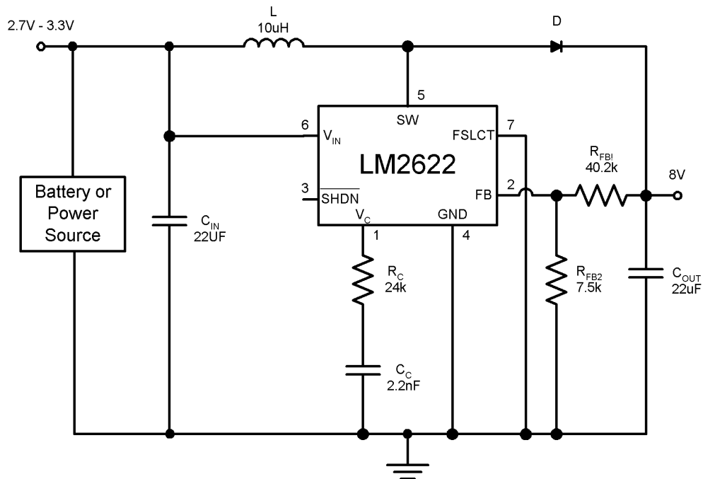
FIGURE 4. 600 kHz operation
