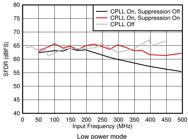
Figure 8-44. SFDR vs F_{IN} and C-PLL modes
