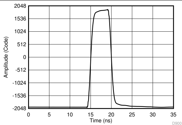
Figure 10-2. Measured Pulse using Sub-Sampling Technique for Equivalent 32 GSPS Measurement
