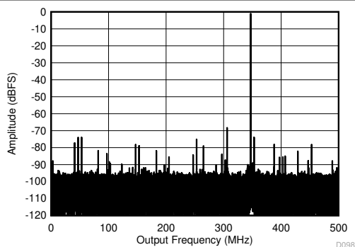
Figure 8-13. Single Tone FFT at 347 MHz and -1 dBFS
