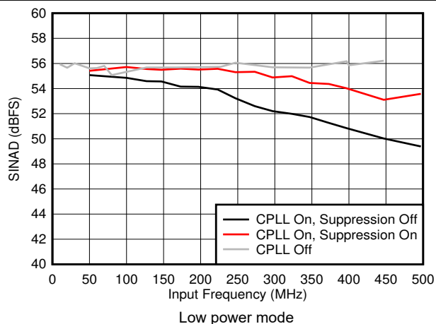
Figure 8-46. SINAD vs F_{IN} and C-PLL modes
