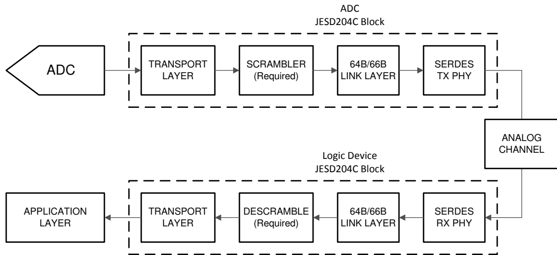
Figure 9-8. Simplified 64B/66B Encoded JESD204C Interface Diagram
