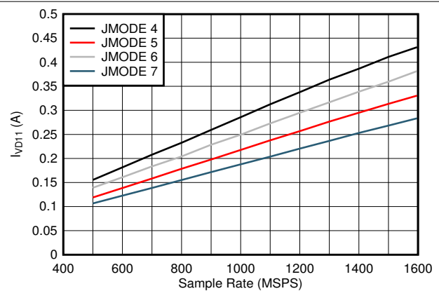
Figure 8-94. Dual Channel, I_{VD11} vs F_s
