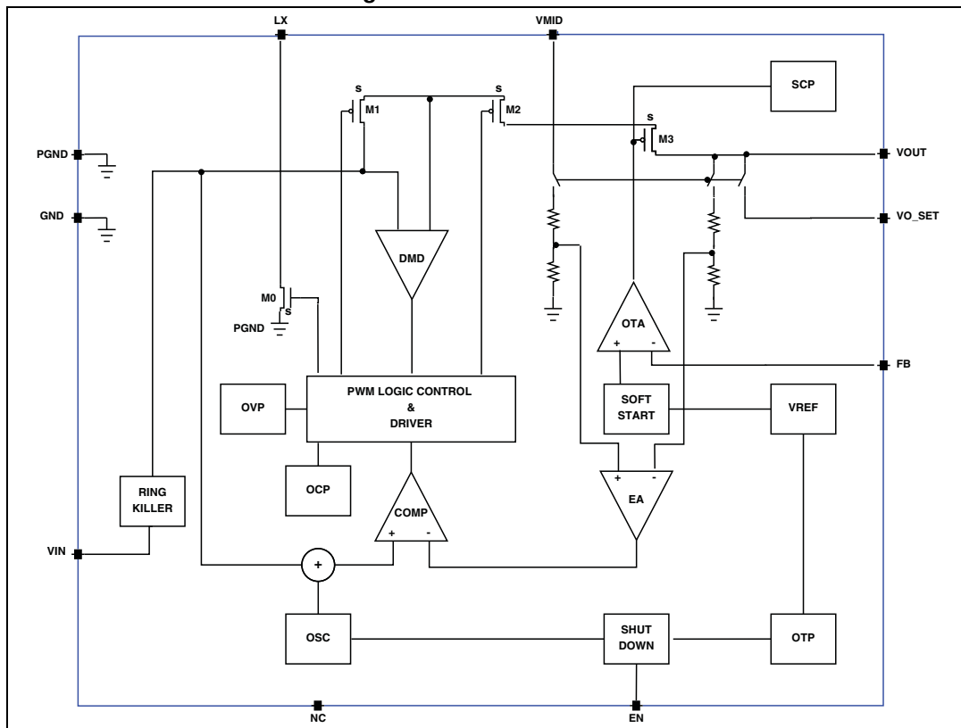
Figure 2. Block schematic
