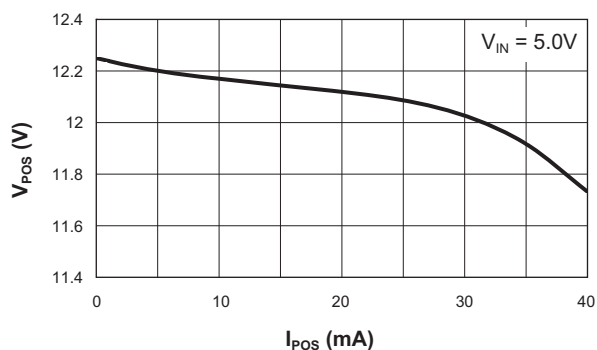
Positive Output Voltage vs. Load Current ( T = 85^{\circ}\text{C} )
