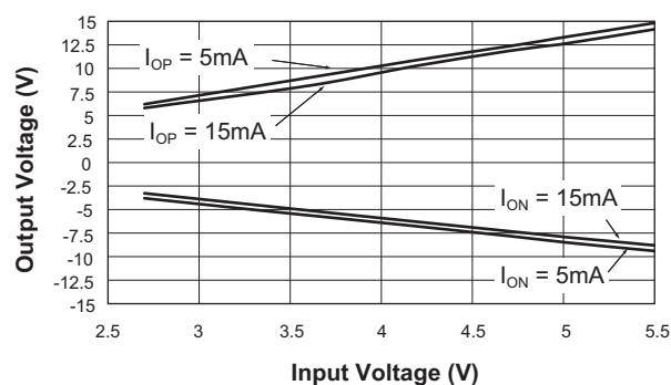
Maximum V_{\text{OUT}} vs. V_{\text{IN}} ( I_{\text{OUT}} = 5\text{mA} and 15\text{mA} )
