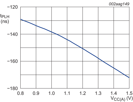
Fig 14. Typical port B to port A propagation delay versus port A supply voltage
