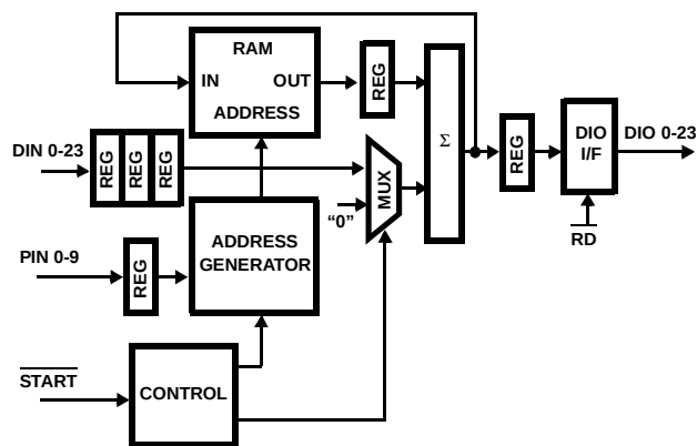
FIGURE 6. BIN ACCUMULATE BLOCK DIAGRAM
