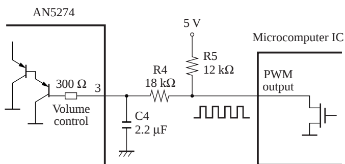
Fig. Volume control interface circuit for AN5274
