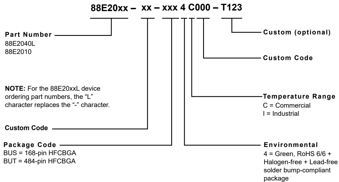
Figure 35: Sample Part Number
