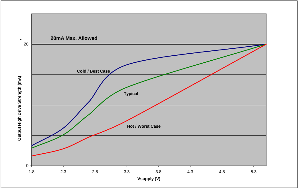
Figure 5. Output High Drive Strength Graph
