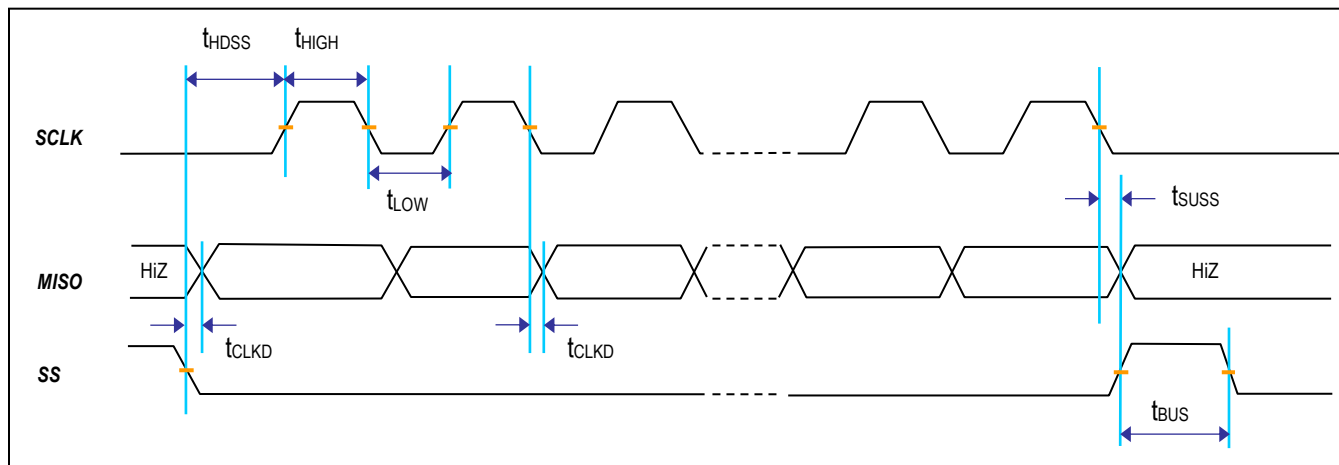
Figure 18. SPI Timing Diagram
