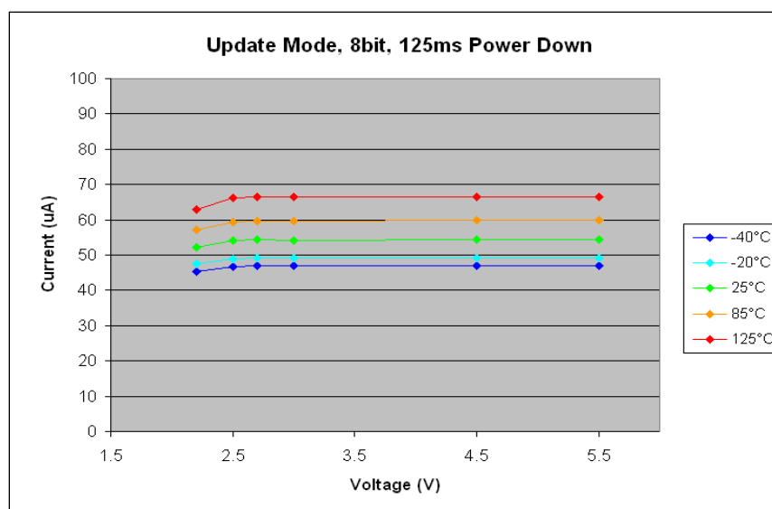
Figure 3. Worst Case Settings (Typical Part)
