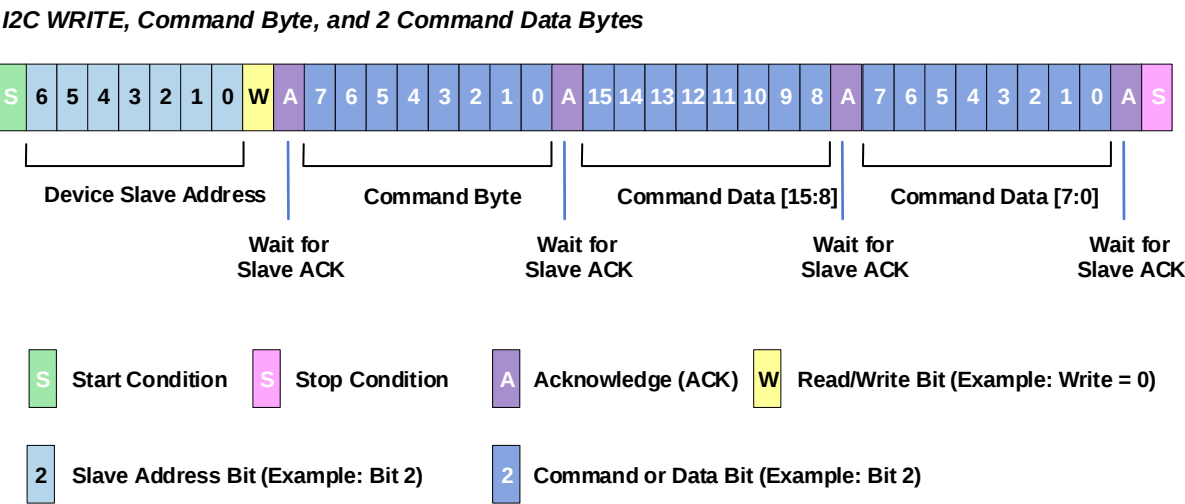
Figure 25. I2C Command Format
