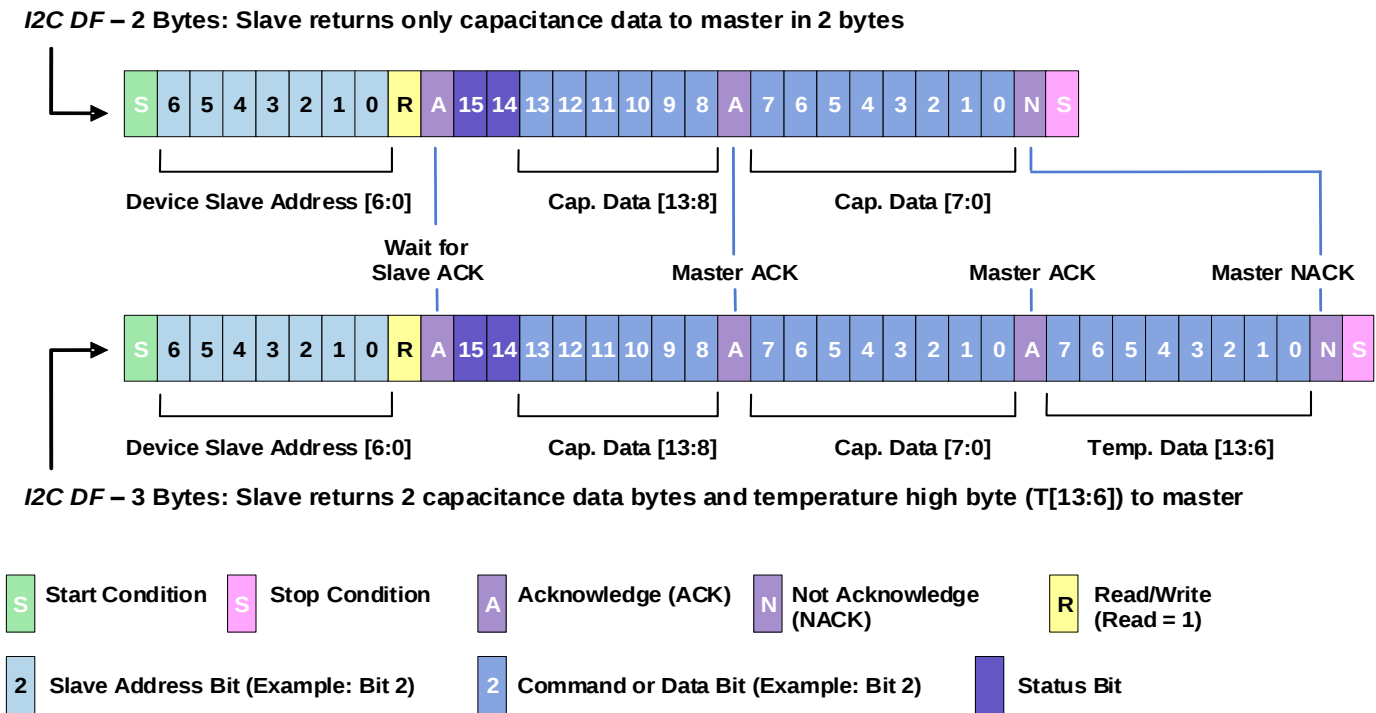
Figure 19. I2C Measurement Packet Reads
