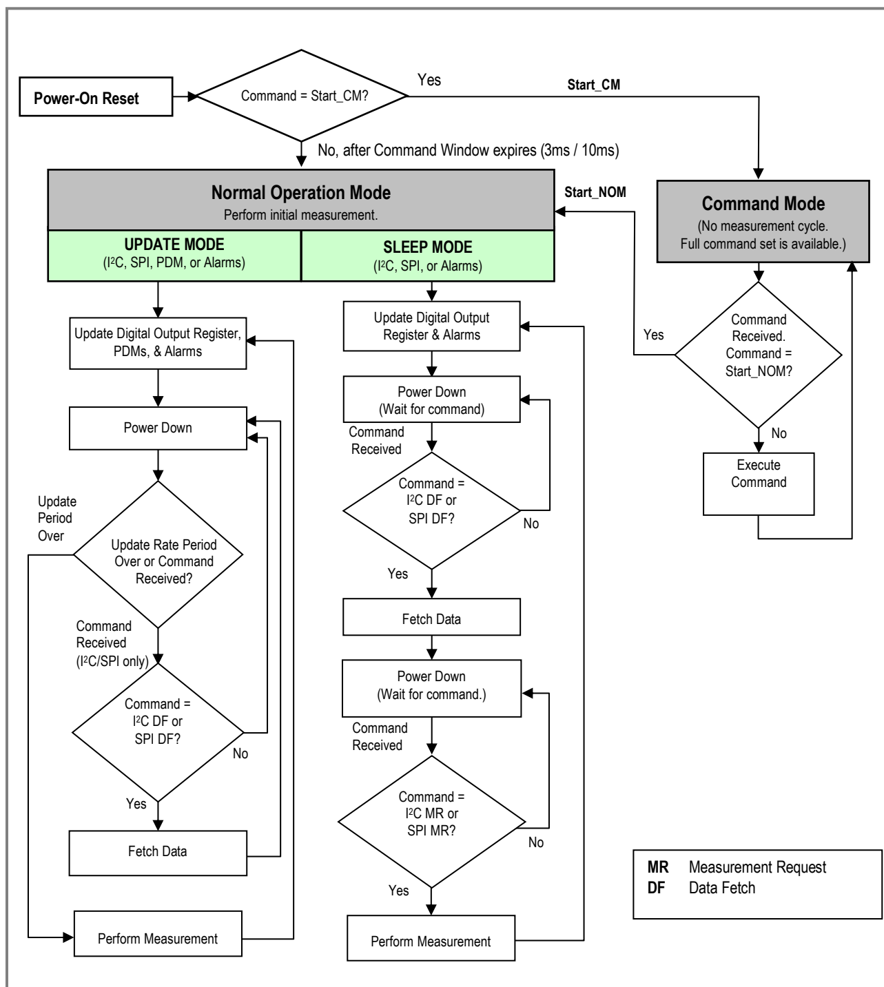
Figure 10. General Operation
