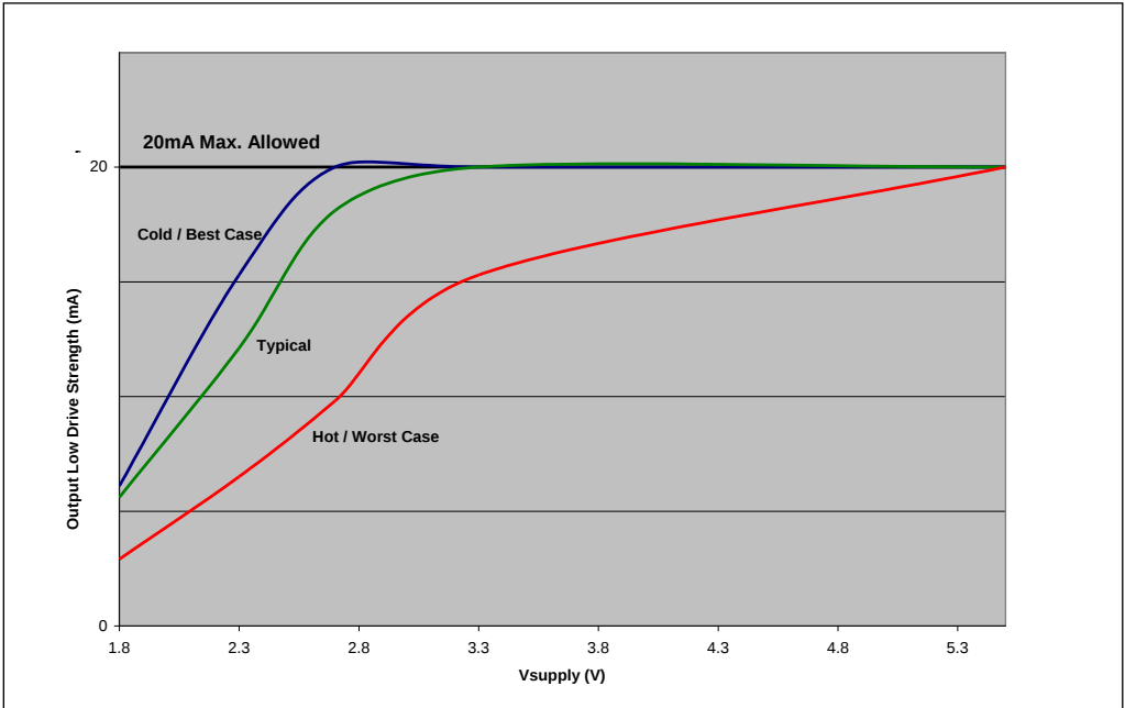
Figure 6. Output Low Drive Strength Graph
