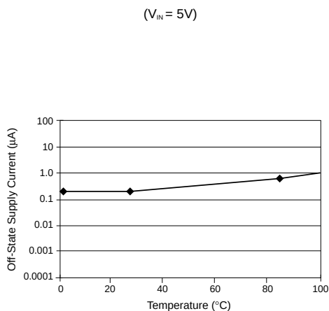
Figure P15. Off-State Supply Current vs. Ambient Temperature
