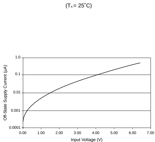
Figure P14. Off-State Supply Current vs. Input Voltage
