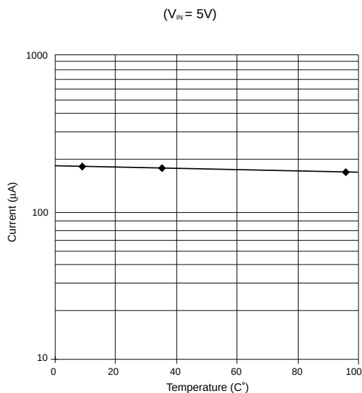
Figure P13. On-State Supply Current vs. Ambient Temperature
