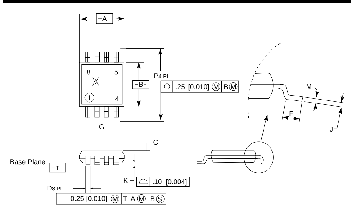
Figure P25. SO-8 Device Dimensions
