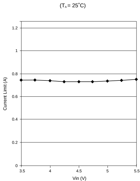
Figure P16. Current Limit vs. Input Voltage
