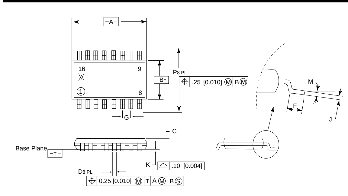
Figure P26. SO-16 Device Dimensions
