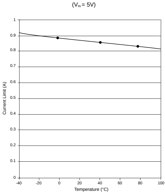
Figure P17. Current Limit vs. Ambient Temperature
