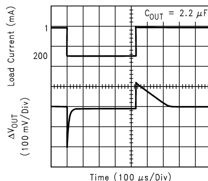
LDO5 (3.0V Option) Load Transient
