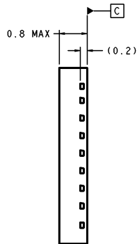
28 Lead LLP Package NS Package Number lqa28A
