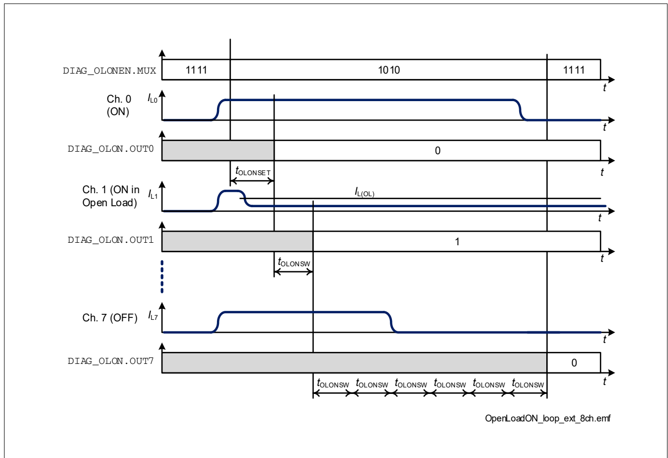
Figure 29 Open Load at ON timings (diagnosis loop - channels driven by micro-controller directly)
