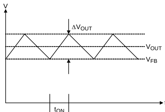
Figure 2. Output Voltage Waveform
