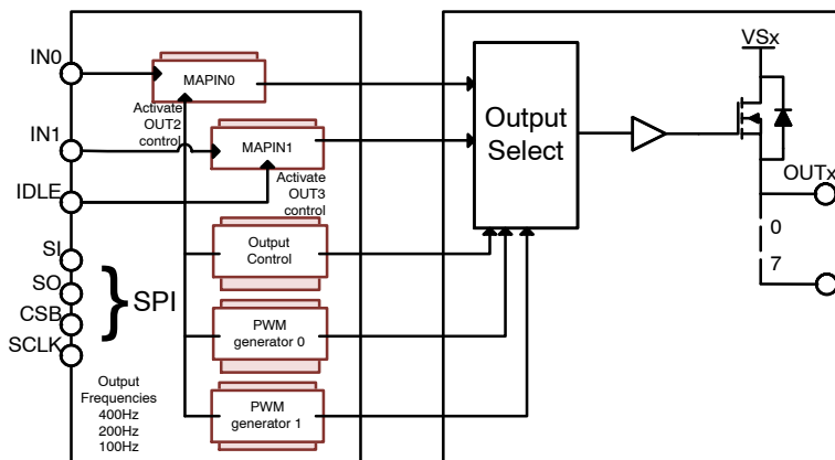
Figure 18. Output Control
