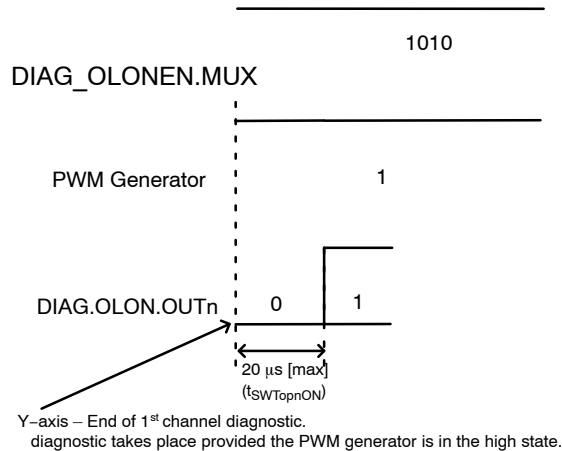
Figure 30. Subsequent Channel Delay Times
