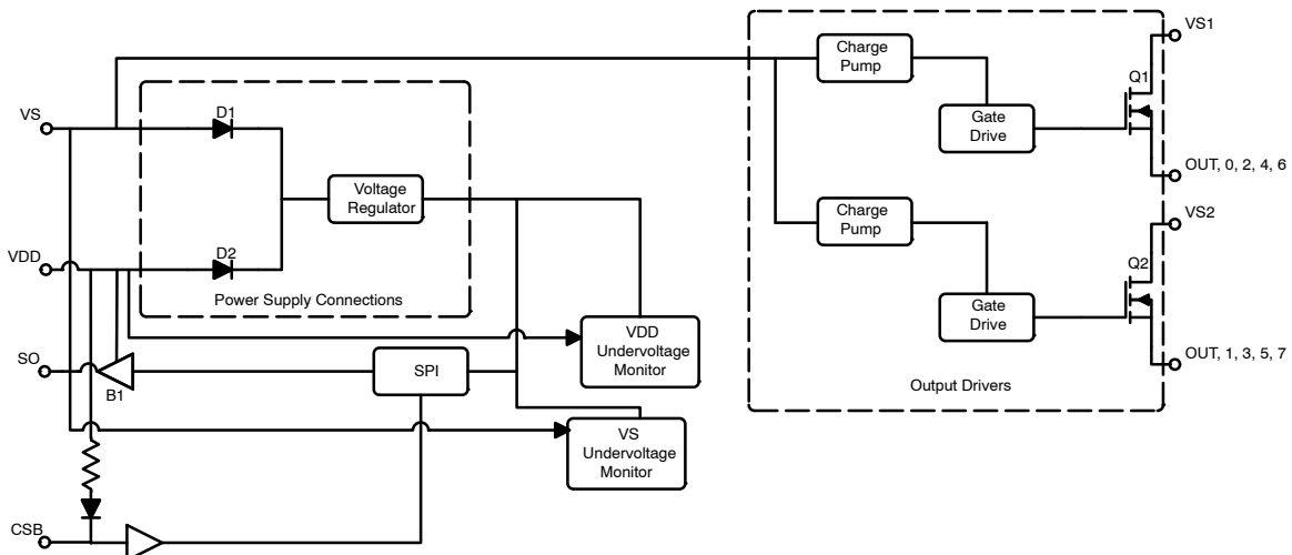
Figure 15. Power Supply
