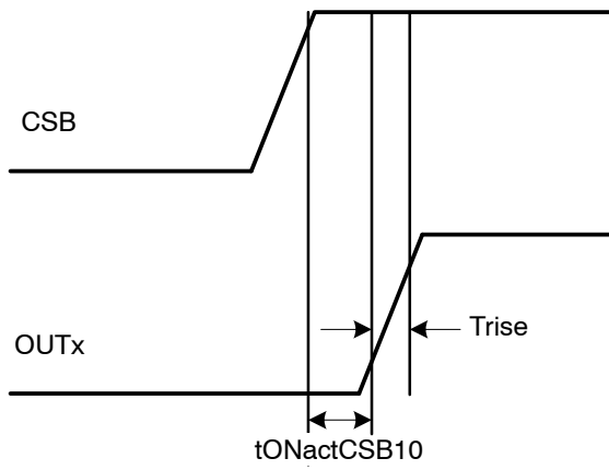
Figure 4. Serial Turn On
