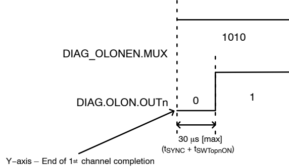
Figure 28. Subsequent Channel Loop Delay Times
