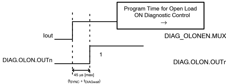
Figure 24. Direct Channel Time for Monitor Active
