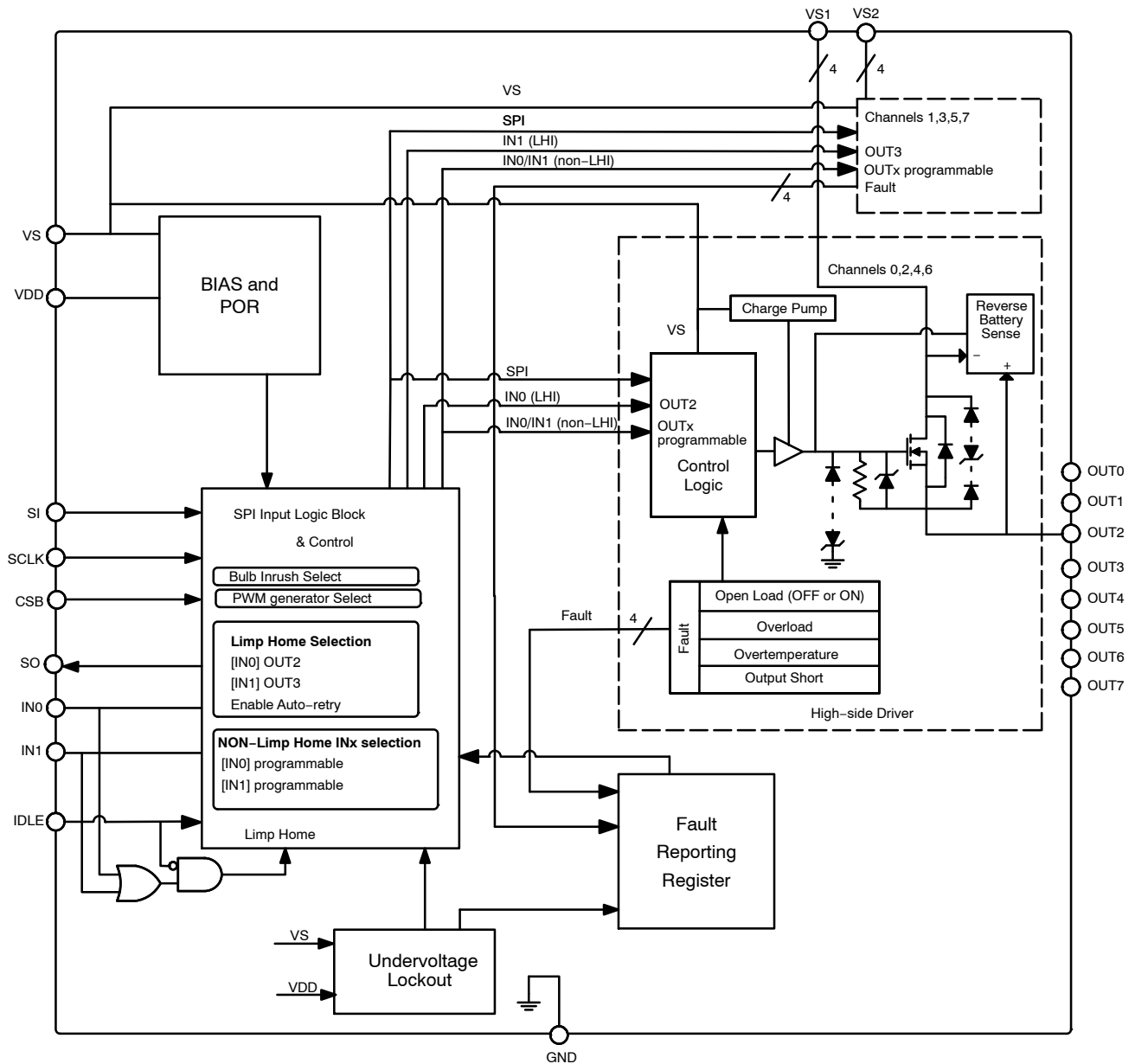
Figure 2. Block Diagram
