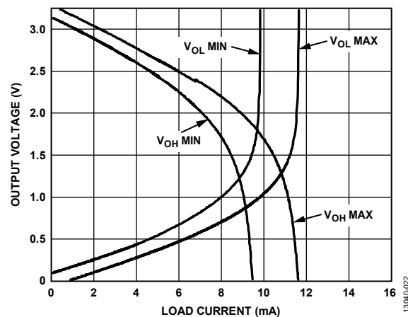
Figure 22. Typical Output Voltage vs. Load Current
