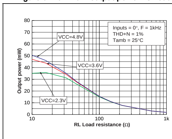
Figure 6. Maximum output power vs. load
