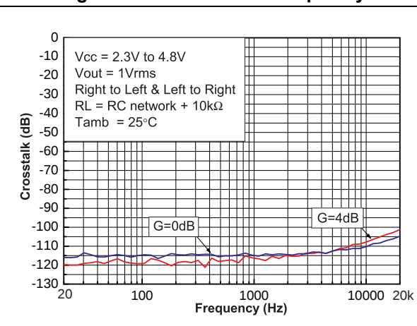
Figure 69. Crosstalk vs. frequency
