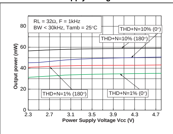
Figure 9. Maximum output power vs. power supply voltage
