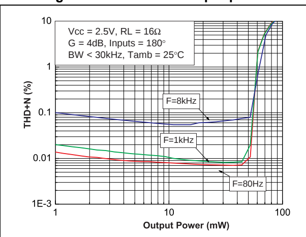
Figure 21. THD+N vs. output power
