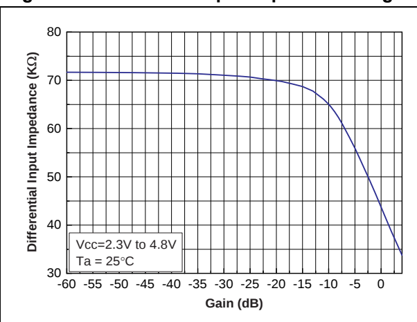
Figure 19. Differential input impedance vs. gain
