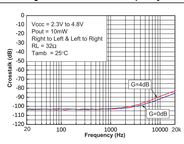
Figure 67. Crosstalk vs. frequency
