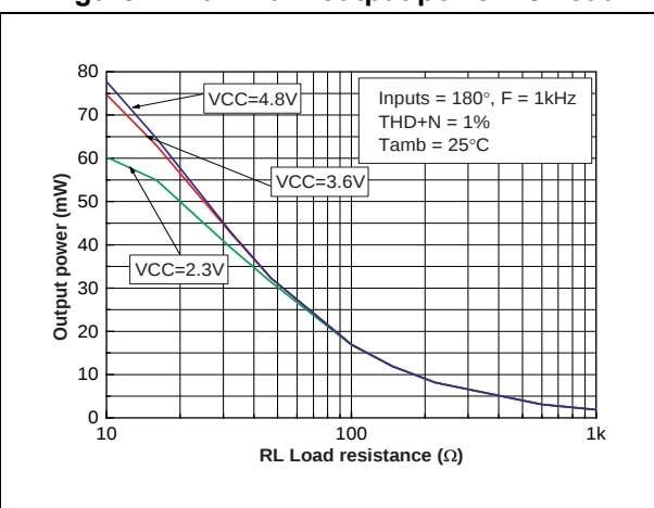
Figure 7. Maximum output power vs. load
