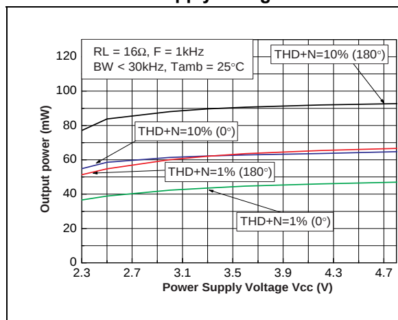
Figure 8. Maximum output power vs. power supply voltage
