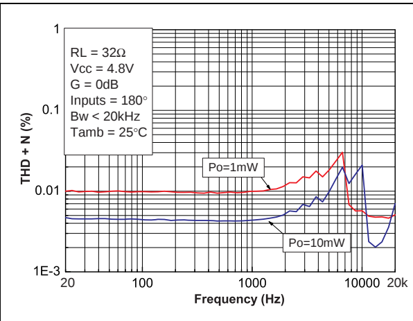
Figure 49. THD+N vs. frequency
