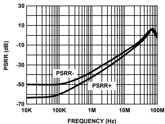
FIGURE 12. POWER SUPPLY REJECTION vs FREQUENCY
