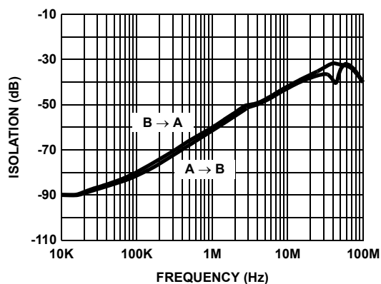
FIGURE 10. CHANNEL ISOLATION vs FREQUENCY
