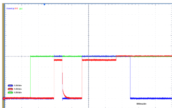
Figure 9. Wake-up pin operation
